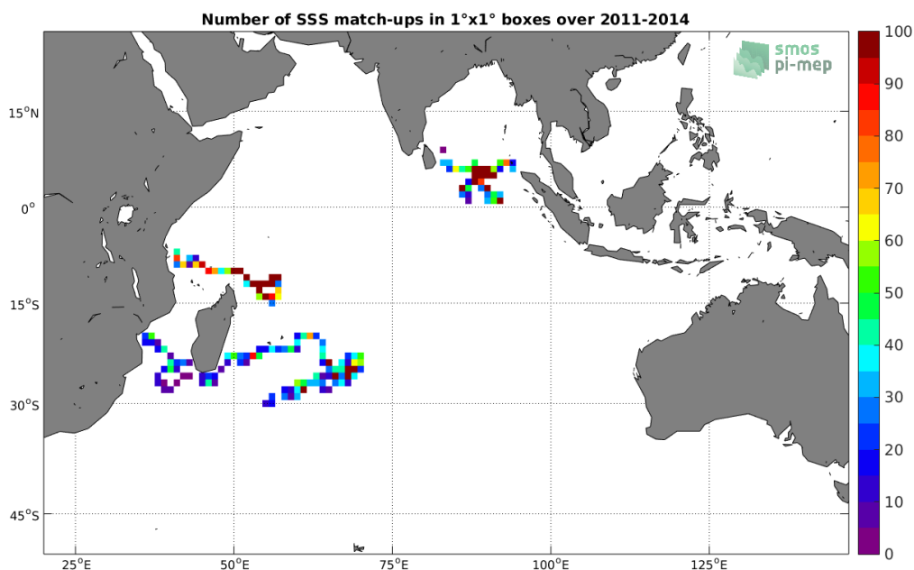
Figure 3: Number of SSS match-ups between Surface drifters SSS and the Aquarius-L4-IPRC-V5-MONTHLY SSS product for the Indian Ocean Pi-MEP region over 1°x1° boxes and for the full satellite product period.
