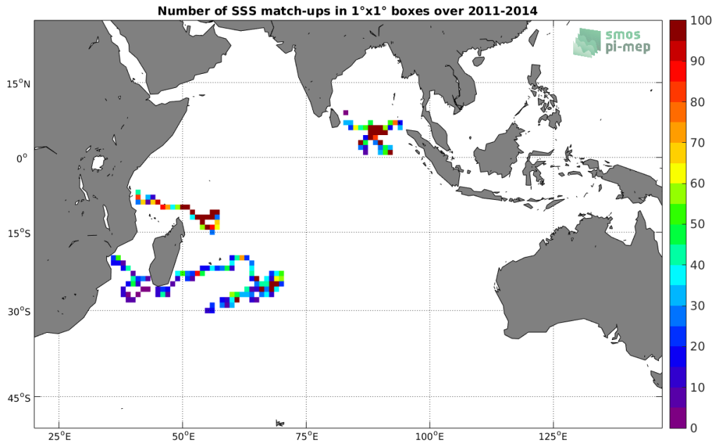
Figure 3: Number of SSS match-ups between Surface drifters SSS and the Aquarius-L4-IPRC-V5-MONTHLY SSS product for the Indian Ocean Pi-MEP region over 1°x1° boxes and for the full satellite product period.
