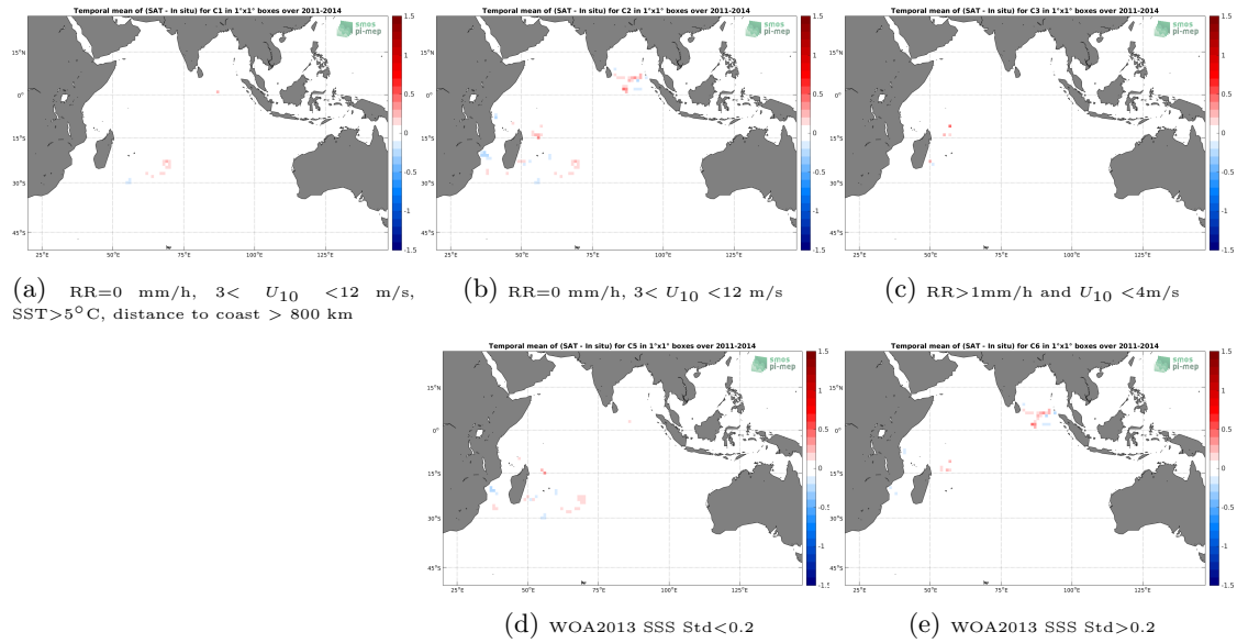
Figure 11: Temporal mean gridded over spatial boxes of size 1^\circ \times 1^\circ of \Delta SSS (Aquarius-L4-IPRC-V5-MONTHLY - Surface drifters) for 5 different subdatasets corresponding to:RR=0 mm/h, 3 < U_{10} < 12 m/s, SST >5^\circ C, distance to coast > 800 km (a), RR=0 mm/h, 3 < U_{10} < 12 m/s (b), RR >1 mm/h and U_{10} < 4 m/s (c), WOA2013 SSS Std <0.2 (d), WOA2013 SSS Std >0.2 (e).
