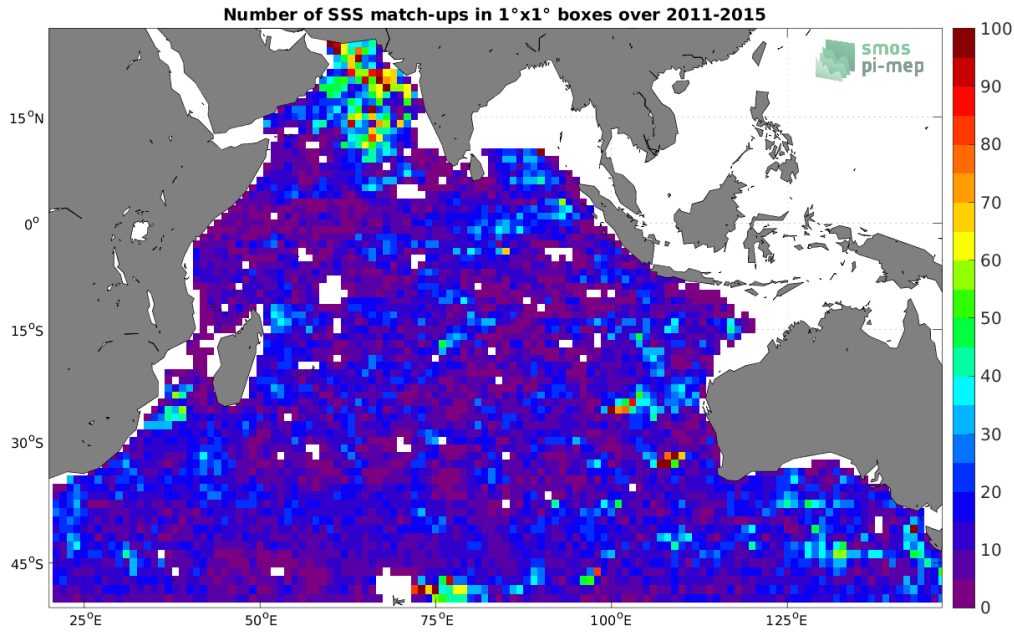
Figure 4: Number of SSS match-ups between Argo SSS and the Aquarius SSS L4 OI v5 - Monthly (IPRC) SSS product for the Indian Ocean Pi-MEP region over 1^\circ \times 1^\circ boxes and for the full satellite product period.
