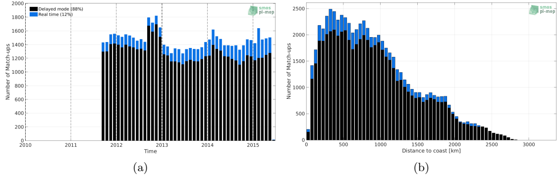
Figure 1: Number of match-ups between Argo and Aquarius SSS L4 OI v5 - Monthly (IPRC) SSS as a function of time (a) and as function of the distance to coast (b) over the Indian Ocean Pi-MEP region and for the full satellite product period.
