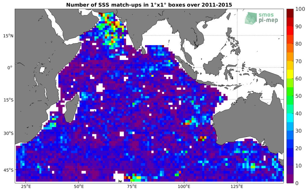
Figure 4: Number of SSS match-ups between Argo SSS and the Aquarius SSS L4 OI v5 - Monthly (IPRC) SSS product for the Indian Ocean Pi-MEP region over 1°x1° boxes and for the full satellite product period.
