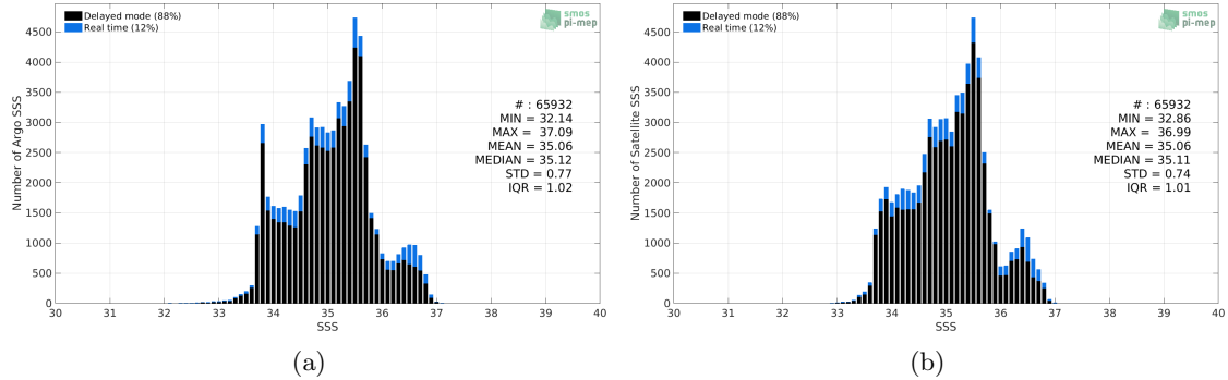
Figure 2: Histograms of SSS from Argo (a) and Aquarius SSS L4 OI v5 - Monthly (IPRC) (b) considering all match-up pairs per bins of 0.1 over the Indian Ocean Pi-MEP region and for the full satellite product period.
