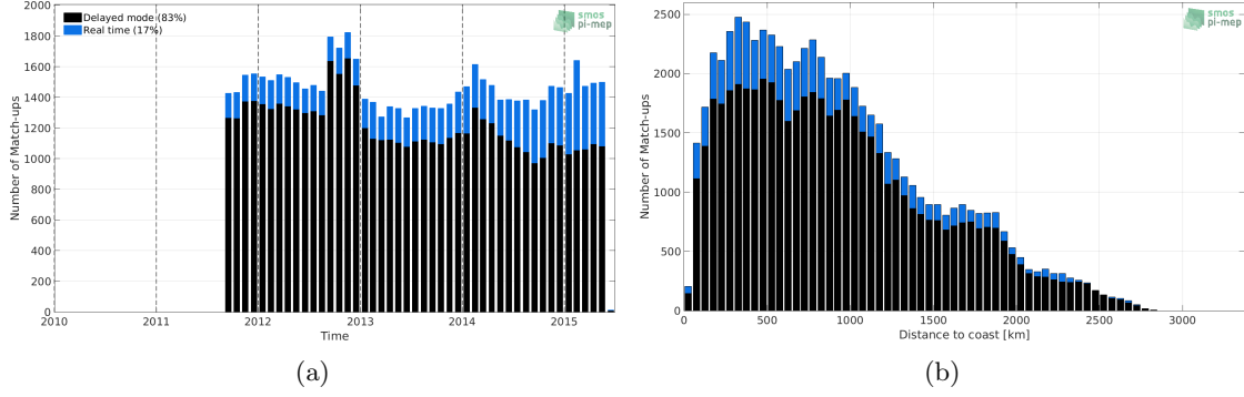
Figure 1: Number of match-ups between Argo and Aquarius-L4-IPRC-V5-MONTHLY SSS as a function of time (a) and as function of the distance to coast (b) over the Indian Ocean Pi-MEP region and for the full satellite product period.
