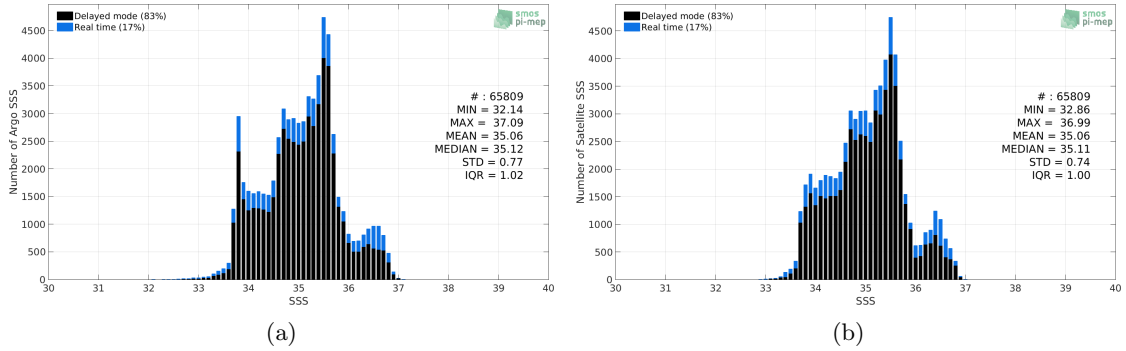
Figure 2: Histograms of SSS from Argo (a) and Aquarius-L4-IPRC-V5-MONTHLY (b) considering all match-up pairs per bins of 0.1 over the Indian Ocean Pi-MEP region and for the full satellite product period.
