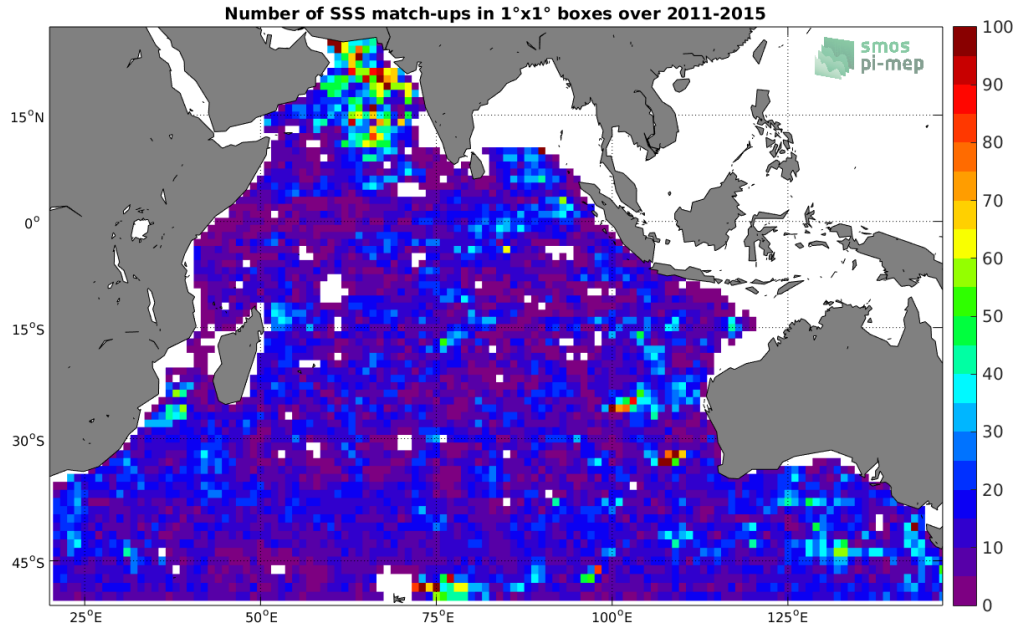
Figure 4: Number of SSS match-ups between Argo SSS and the Aquarius-L4-IPRC-V5-MONTHLY SSS product for the Indian Ocean Pi-MEP region over 1^\circ \times 1^\circ boxes and for the full satellite product period.
