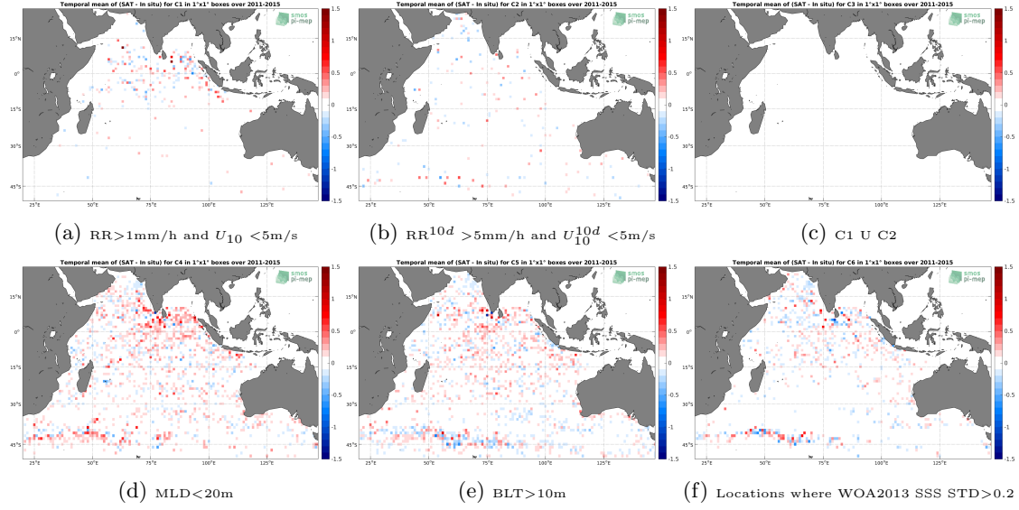
Figure 12: Temporal mean gridded over spatial boxes of size 1^\circ \times 1^\circ of \Delta\text{SSS} (Aquarius-L4-IPRC-V5-MONTHLY - Argo) for 6 different subdatasets corresponding to: \text{RR} > 1\text{mm/h} and U_{10} < 5\text{m/s} (a), \text{RR}^{10d} > 5\text{mm/h} and U_{10}^{10d} < 5\text{m/s} (b), C1 U C2 (c), \text{MLD} < 20\text{m} (d), \text{BLT} > 10\text{m} (e), Locations where WOA2013 SSS STD > 0.2 (f).
