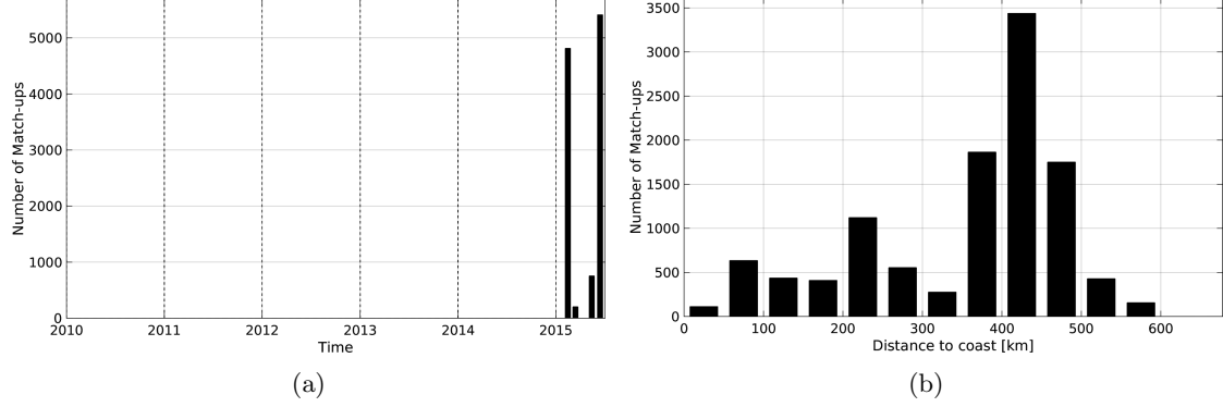
Figure 1: Number of match-ups between TSG-SAMOS and Aquarius-L4-IPRC-V4-WEEKLY SSS as a function of time (a) and as function of the distance to coast (b) over the Indian Ocean Pi-MEP region and for the full satellite product period.
