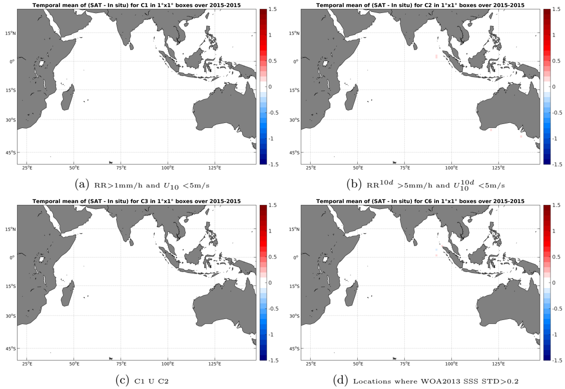
Figure 12: Temporal mean gridded over spatial boxes of size 1^\circ \times 1^\circ of \Delta SSS (Aquarius-L4-IPRC-V4-WEEKLY - TSG-SAMOS) for 4 different subdatasets corresponding to: RR > 1 mm/h and U_{10} < 5 m/s (a), RR^{10d} > 5 mm/h and U_{10}^{10d} < 5 m/s (b), C1 U C2 (c), Locations where WOA2013 SSS STD > 0.2 (d).
