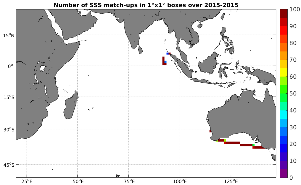
Figure 4: Number of SSS match-ups between TSG-SAMOS SSS and the Aquarius-L4-IPRC-V4-WEEKLY SSS product for the Indian Ocean Pi-MEP region over 1^\circ \times 1^\circ boxes and for the full satellite product period.
