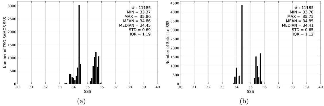
Figure 2: Histograms of SSS from TSG-SAMOS (a) and Aquarius-L4-IPRC-V4-WEEKLY (b) considering all match-up pairs per bins of 0.1 over the Indian Ocean Pi-MEP region and for the full satellite product period.
