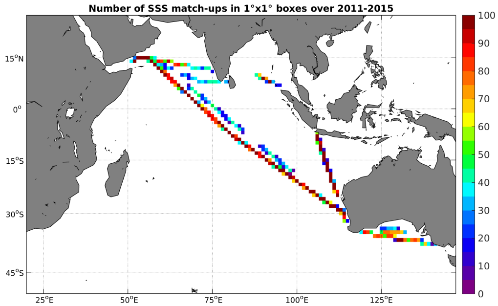
Figure 4: Number of SSS match-ups between TSG-LEGOS-DM SSS and the Aquarius-L4-IPRC-V4-WEEKLY SSS product for the Indian Ocean Pi-MEP region over 1^\circ \times 1^\circ boxes and for the full satellite product period.
