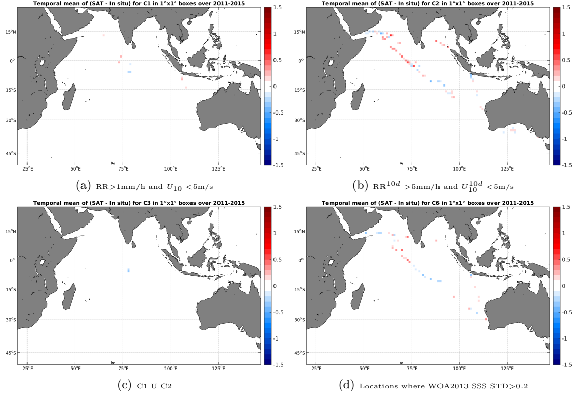
Figure 12: Temporal mean gridded over spatial boxes of size 1^\circ \times 1^\circ of \Delta SSS (Aquarius-L4-IPRC-V4-WEEKLY - TSG-LEGOS-DM) for 4 different subdatasets corresponding to: RR > 1 mm/h and U_{10} < 5 m/s (a), RR^{10d} > 5 mm/h and U_{10}^{10d} < 5 m/s (b), C1 U C2 (c), Locations where WOA2013 SSS STD > 0.2 (d).
