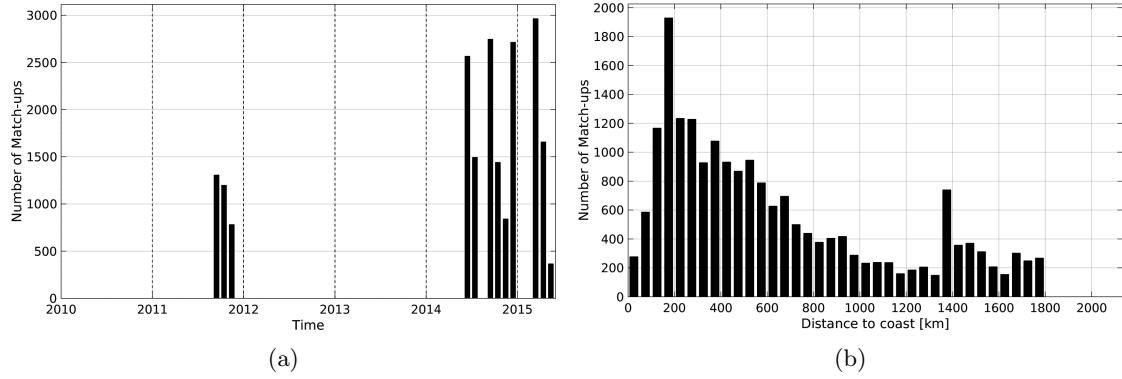
Figure 1: Number of match-ups between TSG-LEGOS-DM and Aquarius-L4-IPRC-V4-WEEKLY SSS as a function of time (a) and as function of the distance to coast (b) over the Indian Ocean Pi-MEP region and for the full satellite product period.
