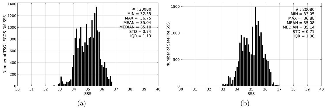
Figure 2: Histograms of SSS from TSG-LEGOS-DM (a) and Aquarius-L4-IPRC-V4-WEEKLY (b) considering all match-up pairs per bins of 0.1 over the Indian Ocean Pi-MEP region and for the full satellite product period.
