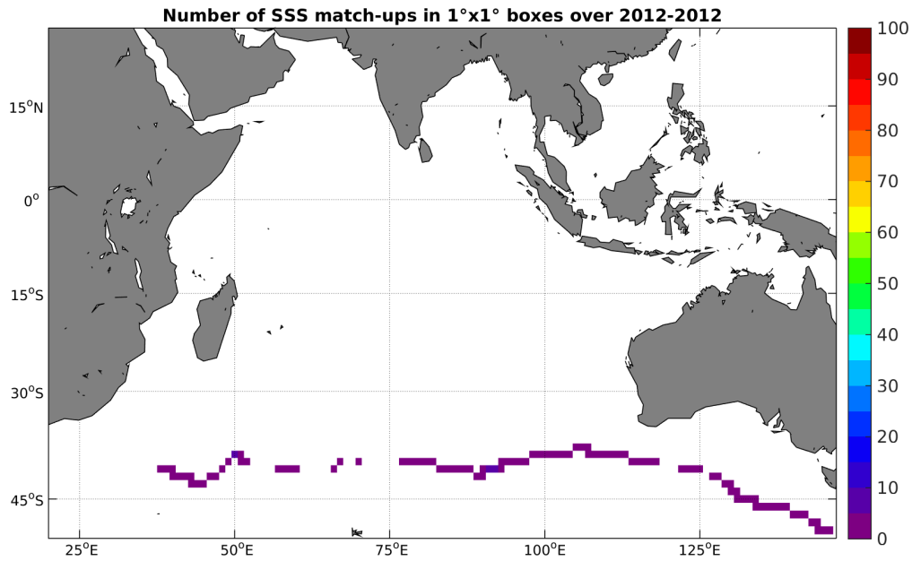
Figure 4: Number of SSS match-ups between TSG-GOSUD-Sailing-ship SSS and the Aquarius-L4-IPRC-V4-WEEKLY SSS product for the Indian Ocean Pi-MEP region over 1^\circ \times 1^\circ boxes and for the full satellite product period.
