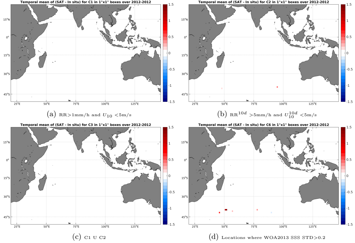
Figure 12: Temporal mean gridded over spatial boxes of size 1^\circ \times 1^\circ of \Delta SSS (Aquarius-L4-IPRC-V4-WEEKLY - TSG-GOSUD-Sailing-ship) for 4 different subdatasets corresponding to: RR > 1\text{mm/h} and U_{10} < 5\text{m/s} (a), RR^{10d} > 5\text{mm/h} and U_{10}^{10d} < 5\text{m/s} (b), C1 U C2 (c), Locations where WOA2013 SSS STD > 0.2 (d).
