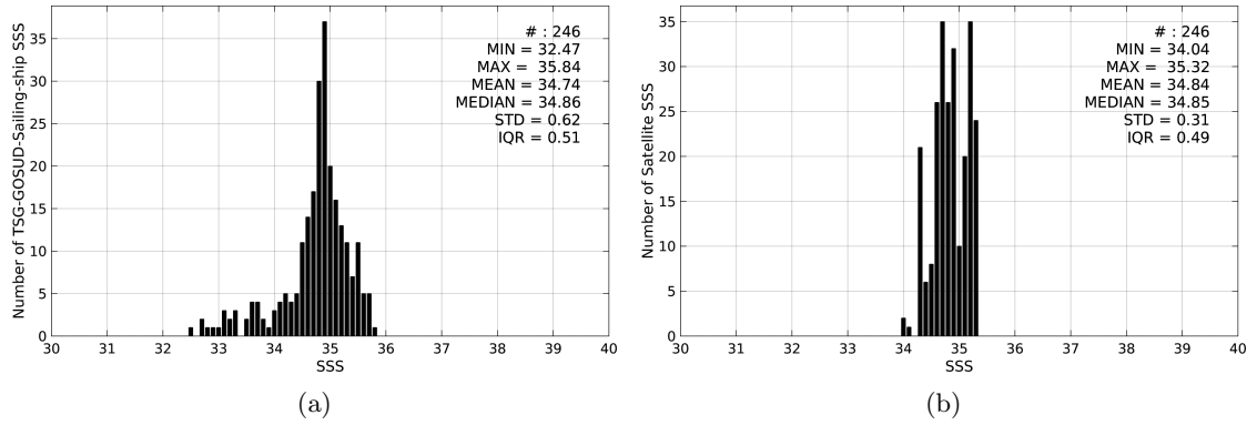
Figure 2: Histograms of SSS from TSG-GOSUD-Sailing-ship (a) and Aquarius-L4-IPRC-V4-WEEKLY (b) considering all match-up pairs per bins of 0.1 over the Indian Ocean Pi-MEP region and for the full satellite product period.
