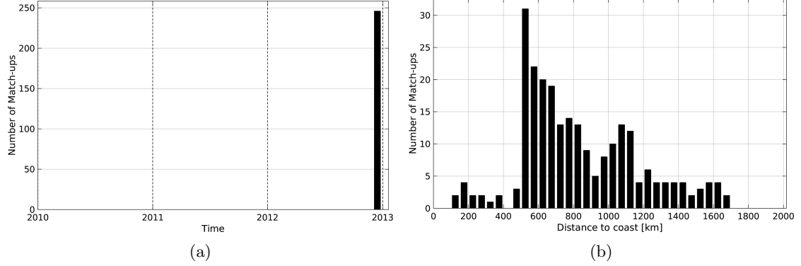
Figure 1: Number of match-ups between TSG-GOSUD-Sailing-ship and Aquarius-L4-IPRC-V4-WEEKLY SSS as a function of time (a) and as function of the distance to coast (b) over the Indian Ocean Pi-MEP region and for the full satellite product period.
