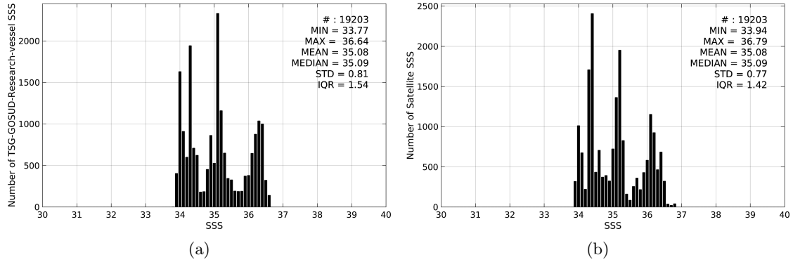
Figure 2: Histograms of SSS from TSG-GOSUD-Research-vessel (a) and Aquarius-L4-IPRC-V4-WEEKLY (b) considering all match-up pairs per bins of 0.1 over the Indian Ocean Pi-MEP region and for the full satellite product period.
