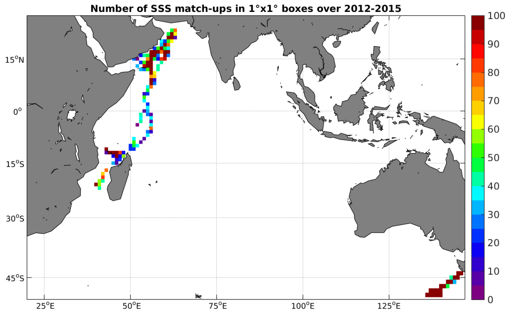
Figure 4: Number of SSS match-ups between TSG-GOSUD-Research-vessel SSS and the Aquarius-L4-IPRC-V4-WEEKLY SSS product for the Indian Ocean Pi-MEP region over 1^\circ \times 1^\circ boxes and for the full satellite product period.
