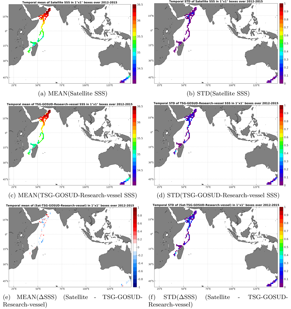
Figure 6: Temporal mean (left) and STD (right) of SSS from Aquarius-L4-IPRC-V4-WEEKLY (top), TSG-GOSUD-Research-vessel (middle), and of \Delta SSS (Satellite - TSG-GOSUD-Research-vessel). Only match-up pairs are used to generate these maps.
