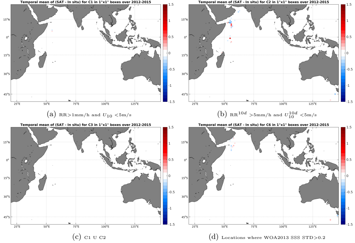
Figure 12: Temporal mean gridded over spatial boxes of size 1^\circ \times 1^\circ of \Delta SSS (Aquarius-L4-IPRC-V4-WEEKLY - TSG-GOSUD-Research-vessel) for 4 different subdatasets corresponding to: RR > 1 mm/h and U_{10} < 5 m/s (a), RR^{10d} > 5 mm/h and U_{10}^{10d} < 5 m/s (b), C1 U C2 (c), Locations where WOA2013 SSS STD > 0.2 (d).
