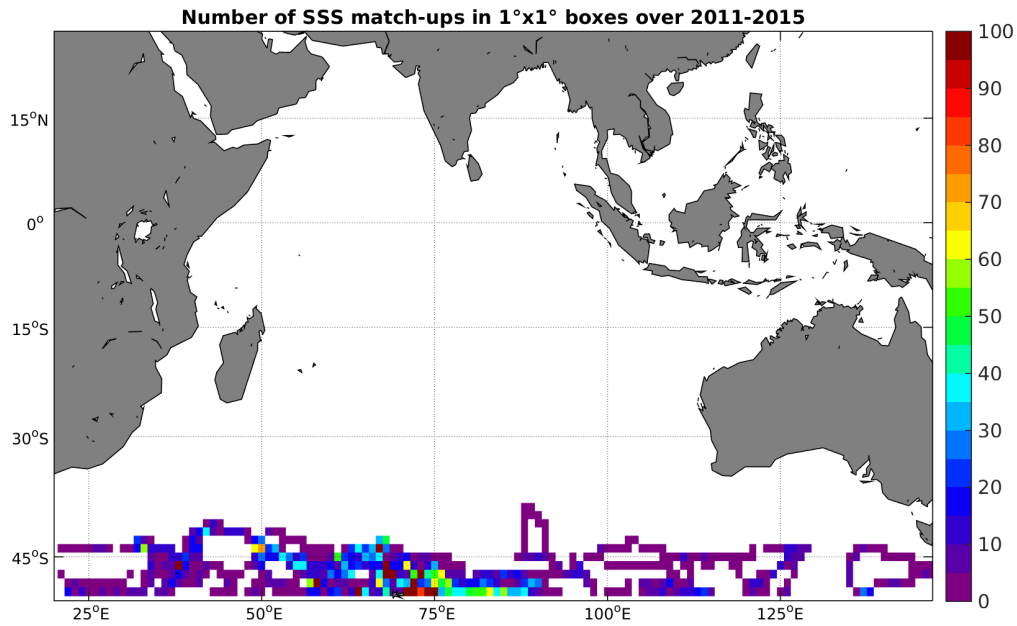
Figure 4: Number of SSS match-ups between Sea mammals SSS and the Aquarius-L4-IPRC-V4-WEEKLY SSS product for the Indian Ocean Pi-MEP region over 1^\circ \times 1^\circ boxes and for the full satellite product period.
