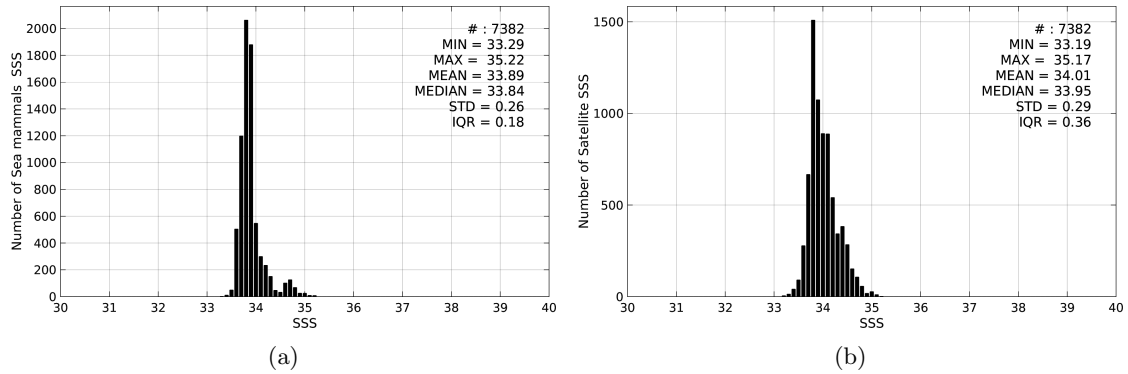
Figure 2: Histograms of SSS from Sea mammals (a) and Aquarius-L4-IPRC-V4-WEEKLY (b) considering all match-up pairs per bins of 0.1 over the Indian Ocean Pi-MEP region and for the full satellite product period.
