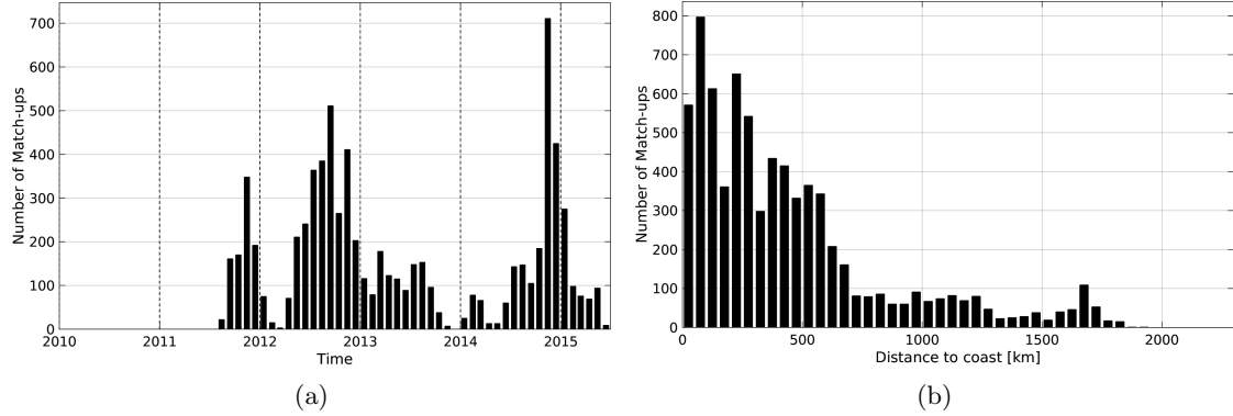
Figure 1: Number of match-ups between Sea mammals and Aquarius-L4-IPRC-V4-WEEKLY SSS as a function of time (a) and as function of the distance to coast (b) over the Indian Ocean Pi-MEP region and for the full satellite product period.
