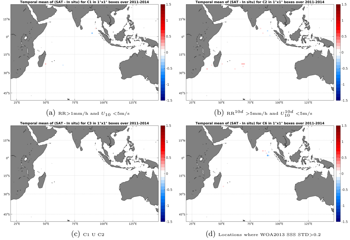
Figure 11: Temporal mean gridded over spatial boxes of size 1^\circ \times 1^\circ of \Delta SSS (Aquarius-L4-IPRC-V4-WEEKLY - Surface drifters) for 4 different subdatasets corresponding to: RR > 1mm/h and U_{10} < 5 m/s (a), RR^{10d} > 5 mm/h and U_{10}^{10d} < 5 m/s (b), C1 U C2 (c), Locations where WOA2013 SSS STD > 0.2 (d).
