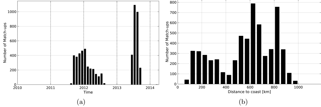
Figure 1: Number of match-ups between Surface drifters and Aquarius-L4-IPRC-V4-WEEKLY SSS as a function of time (a) and as function of the distance to coast (b) over the Indian Ocean Pi-MEP region and for the full satellite product period.
