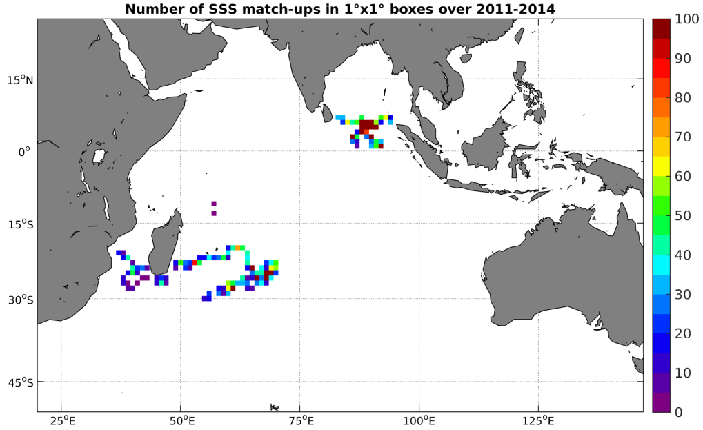
Figure 3: Number of SSS match-ups between Surface drifters SSS and the Aquarius-L4-IPRC-V4-WEEKLY SSS product for the Indian Ocean Pi-MEP region over 1^\circ \times 1^\circ boxes and for the full satellite product period.
