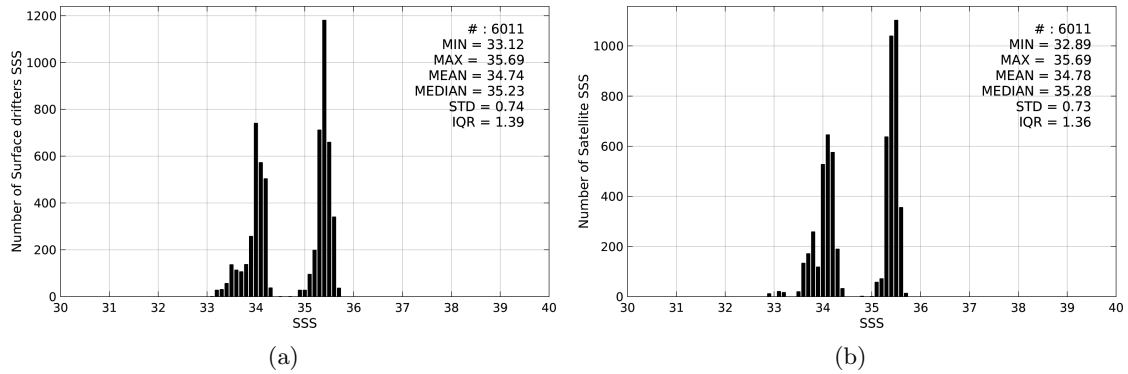
Figure 2: Histograms of SSS from Surface drifters (a) and Aquarius-L4-IPRC-V4-WEEKLY (b) considering all match-up pairs per bins of 0.1 over the Indian Ocean Pi-MEP region and for the full satellite product period.
