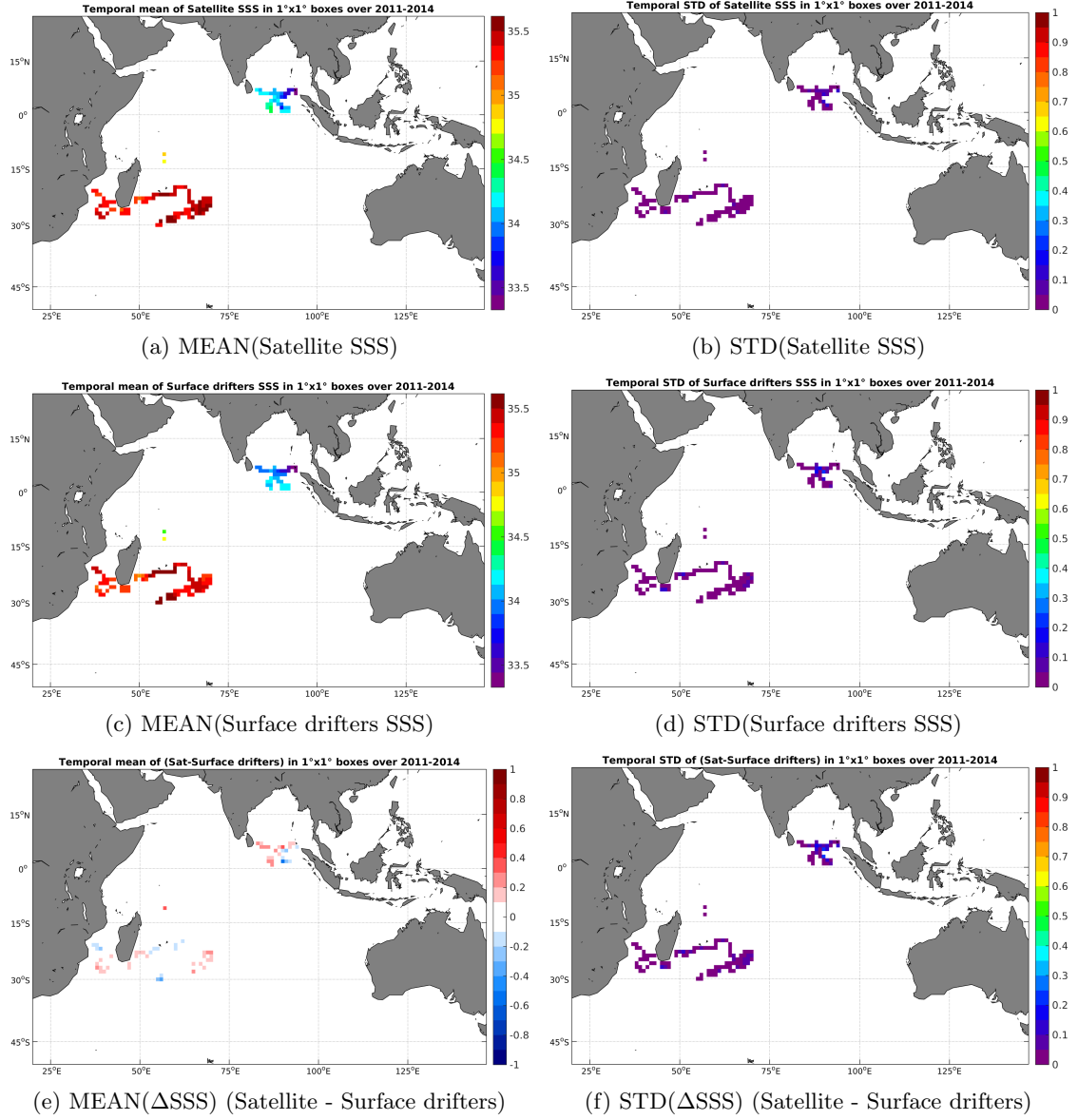
Figure 5: Temporal mean (left) and STD (right) of SSS from Aquarius-L4-IPRC-V4-WEEKLY (top), Surface drifters (middle), and of \Delta SSS (Satellite - Surface drifters). Only match-up pairs are used to generate these maps.
