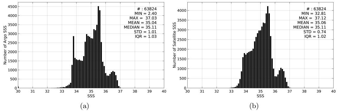
Figure 2: Histograms of SSS from Argo (a) and Aquarius-L4-IPRC-V4-WEEKLY (b) considering all match-up pairs per bins of 0.1 over the Indian Ocean Pi-MEP region and for the full satellite product period.
