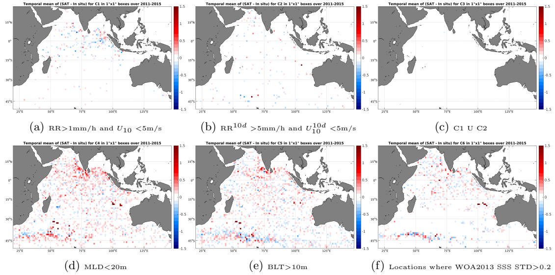
Figure 12: Temporal mean gridded over spatial boxes of size 1^\circ \times 1^\circ of \Delta SSS (Aquarius-L4-IPRC-V4-WEEKLY - Argo) for 6 different subdatasets corresponding to: RR > 1\text{mm/h} and U_{10} < 5\text{m/s} (a), RR^{10d} > 5\text{mm/h} and U_{10}^{10d} < 5\text{m/s} (b), C1 U C2 (c), MLD < 20\text{m} (d), BLT > 10\text{m} (e), Locations where WOA2013 SSS STD > 0.2 (f).
