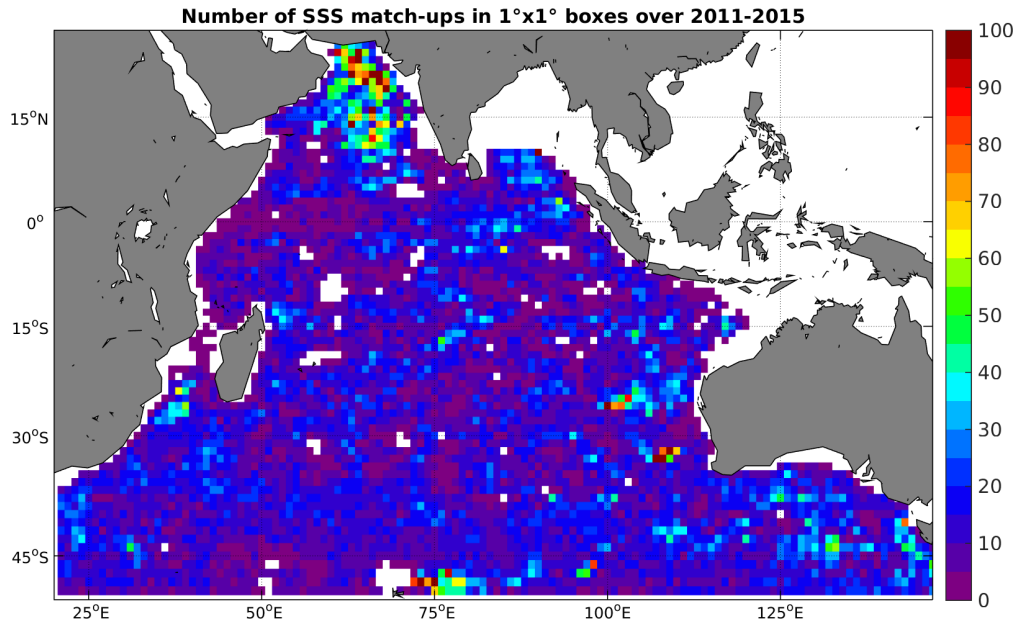
Figure 4: Number of SSS match-ups between Argo SSS and the Aquarius-L4-IPRC-V4-WEEKLY SSS product for the Indian Ocean Pi-MEP region over 1^\circ \times 1^\circ boxes and for the full satellite product period.
