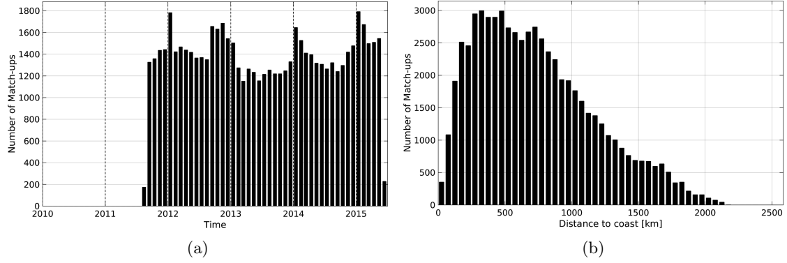
Figure 1: Number of match-ups between Argo and Aquarius-L4-IPRC-V4-WEEKLY SSS as a function of time (a) and as function of the distance to coast (b) over the Indian Ocean Pi-MEP region and for the full satellite product period.
