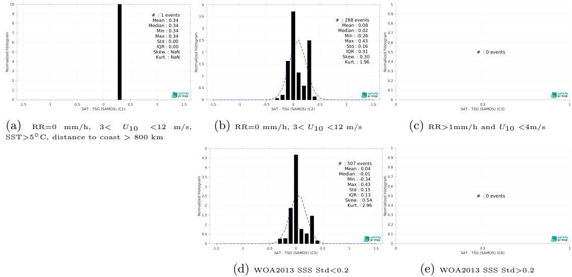
Figure 15: Normalized histogram of \Delta SSS (Aquarius SSS L3 OR v5 - 7-Day running (NASA-GSFC) - TSG (SAMOS)) for 5 different subdatasets corresponding to: RR=0 mm/h, 3 < U_{10} < 12 m/s, SST > 5°C, distance to coast > 800 km (a), RR=0 mm/h, 3 < U_{10} < 12 m/s (b), RR > 1mm/h and U_{10} < 4 m/s (c), WOA2013 SSS Std < 0.2 (d), WOA2013 SSS Std > 0.2 (e).
