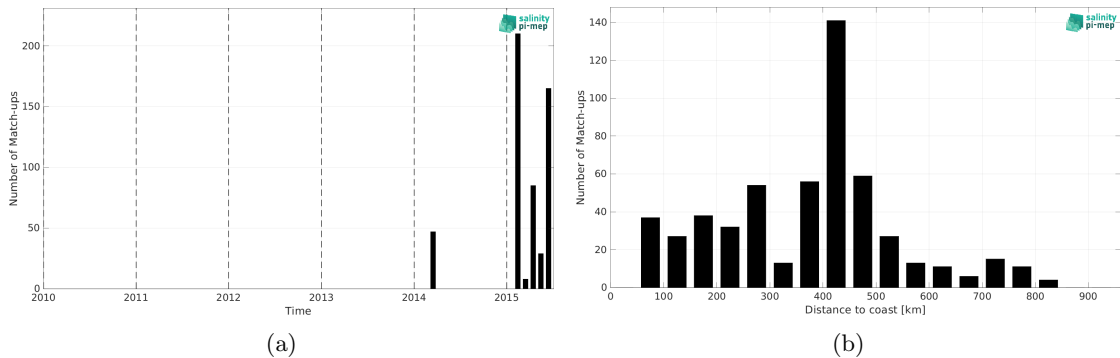
Figure 2: Number of match-ups between TSG (SAMOS) and Aquarius SSS L3 OR v5 - 7-Day running (NASA-GSFC) SSS as a function of time (a) and as function of the distance to coast (b) over the Indian Ocean Pi-MEP region and for the full satellite product period.
