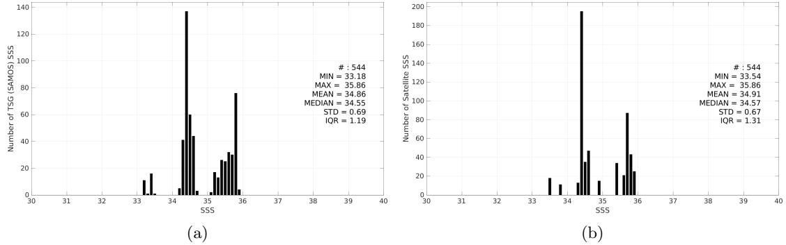
Figure 3: Histograms of SSS from TSG (SAMOS) (a) and Aquarius SSS L3 OR v5 - 7-Day running (NASA-GSFC) (b) considering all match-up pairs per bins of 0.1 over the Indian Ocean Pi-MEP region and for the full satellite product period.
