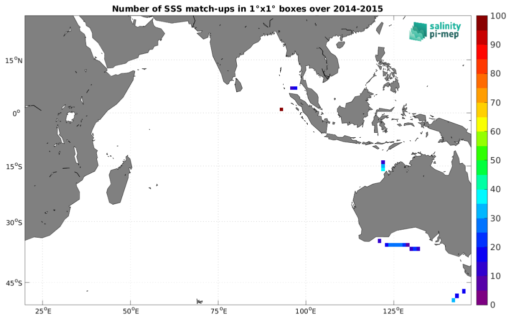
Figure 5: Number of SSS match-ups between TSG (SAMOS) SSS and the Aquarius SSS L3 OR v5 - 7-Day running (NASA-GSFC) SSS product for the Indian Ocean Pi-MEP region over 1^\circ \times 1^\circ boxes and for the full satellite product period.
