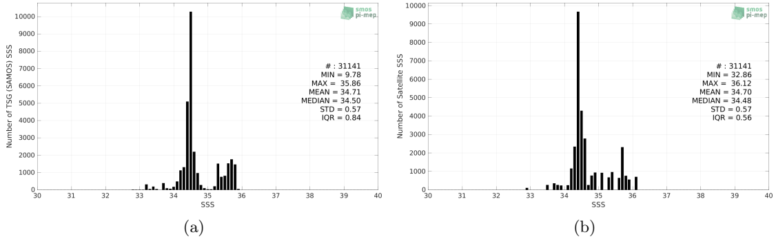
Figure 2: Histograms of SSS from TSG (SAMOS) (a) and Aquarius SSS L3 OR v5 - 7-Day running (NASA-GSFC) (b) considering all match-up pairs per bins of 0.1 over the Indian Ocean Pi-MEP region and for the full satellite product period.
