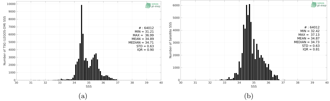
Figure 2: Histograms of SSS from TSG (LEGOS-DM) (a) and Aquarius SSS L3 OR v5 - 7-Day running (NASA-GSFC) (b) considering all match-up pairs per bins of 0.1 over the Indian Ocean Pi-MEP region and for the full satellite product period.
