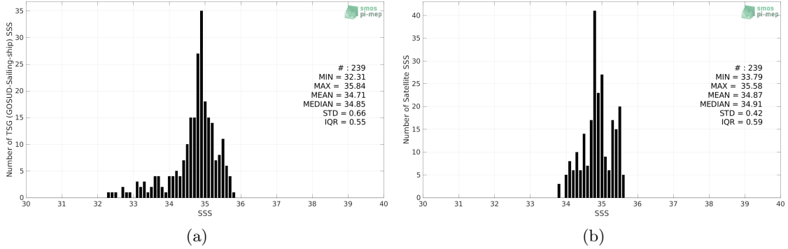
Figure 2: Histograms of SSS from TSG (GOSUD-Sailing-ship) (a) and Aquarius SSS L3 OR v5 - 7-Day running (NASA-GSFC) (b) considering all match-up pairs per bins of 0.1 over the Indian Ocean Pi-MEP region and for the full satellite product period.
