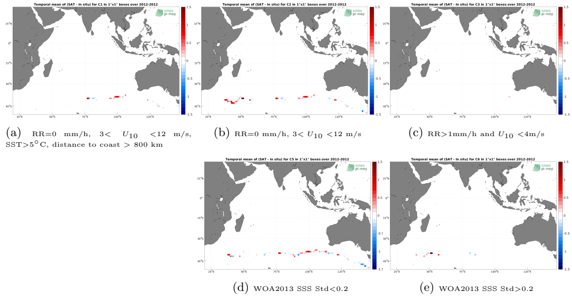
Figure 12: Temporal mean gridded over spatial boxes of size 1^{\circ}\times 1^{\circ} of \Delta SSS (Aquarius SSS L3 OR v5 - 7-Day running (NASA-GSFC) - TSG (GOSUD-Sailing-ship)) for 5 different subdatasets corresponding to:RR=0 mm/h, 3 < U_{10} < 12 m/s, SST >5^{\circ}\text{C} , distance to coast > 800 km (a), RR=0 mm/h, 3 < U_{10} < 12 m/s (b), RR >1 mm/h and U_{10} < 4 m/s (c), WOA2013 SSS Std <0.2 (d), WOA2013 SSS Std >0.2 (e).
