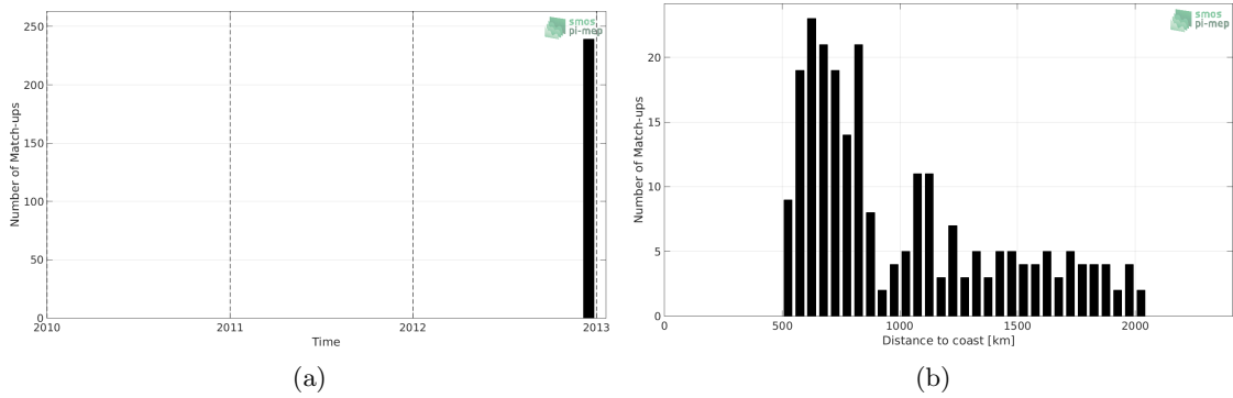
Figure 1: Number of match-ups between TSG-GOSUD-Sailing-ship and Aquarius-L3-OR-V5-7DAY-RUNNING-1DEG SSS as a function of time (a) and as function of the distance to coast (b) over the Indian Ocean Pi-MEP region and for the full satellite product period.
