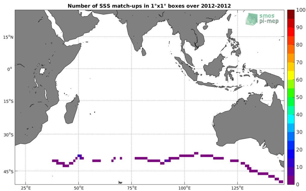
Figure 4: Number of SSS match-ups between TSG-GOSUD-Sailing-ship SSS and the Aquarius-L3-OR-V5-7DAY-RUNNING-1DEG SSS product for the Indian Ocean Pi-MEP region over 1^\circ \times 1^\circ boxes and for the full satellite product period.
