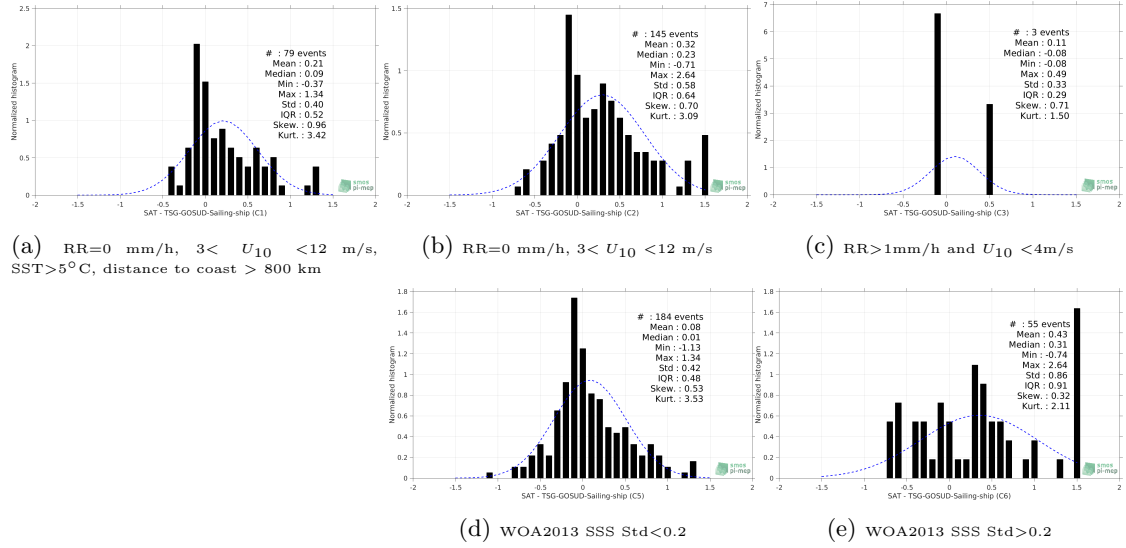
Figure 13: Normalized histogram of \Delta SSS (Aquarius-L3-OR-V5-7DAY-RUNNING-1DEG - TSG-GOSUD-Sailing-ship) for 5 different subdatasets corresponding to: RR=0 mm/h, 3 < U_{10} < 12 m/s, SST > 5°C, distance to coast > 800 km (a), RR=0 mm/h, 3 < U_{10} < 12 m/s (b), RR > 1mm/h and U_{10} < 4 m/s (c), WOA2013 SSS Std < 0.2 (d), WOA2013 SSS Std > 0.2 (e).
