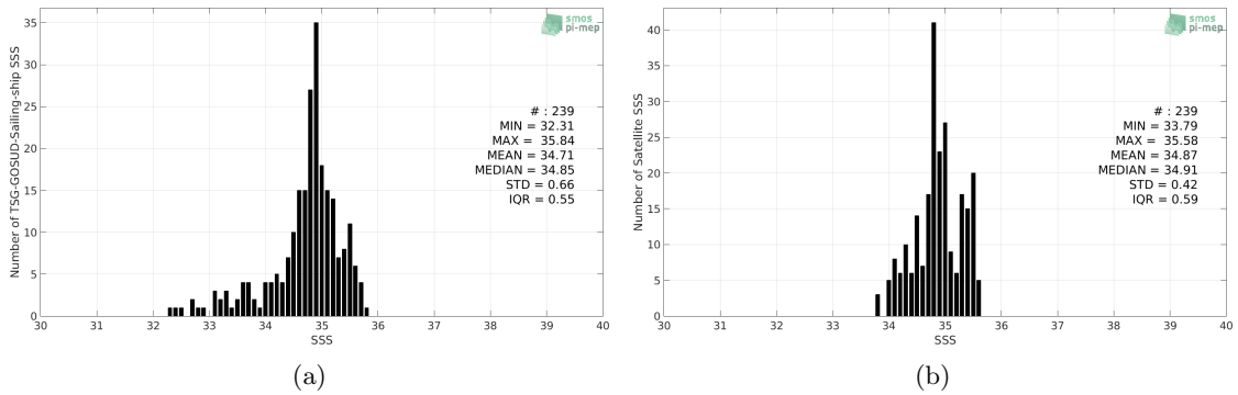
Figure 2: Histograms of SSS from TSG-GOSUD-Sailing-ship (a) and Aquarius-L3-OR-V5-7DAY-RUNNING-1DEG (b) considering all match-up pairs per bins of 0.1 over the Indian Ocean Pi-MEP region and for the full satellite product period.
