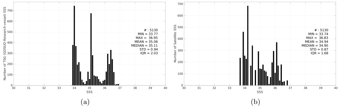
Figure 3: Histograms of SSS from TSG (GOSUD-Research-vessel) (a) and Aquarius SSS L3 OR v5 - 7-Day running (NASA-GSFC) (b) considering all match-up pairs per bins of 0.1 over the Indian Ocean Pi-MEP region and for the full satellite product period.
