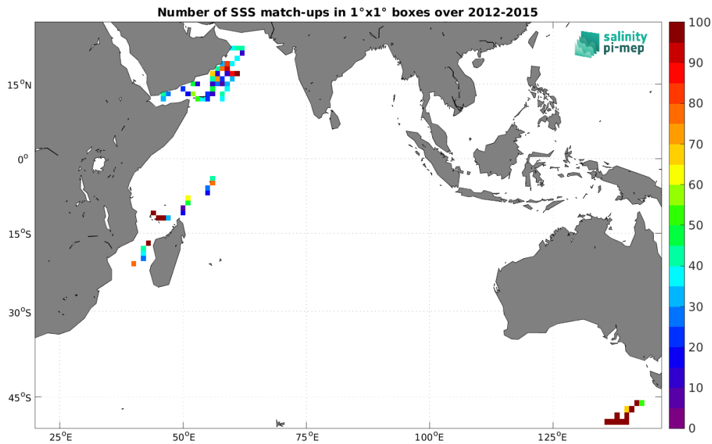
Figure 5: Number of SSS match-ups between TSG (GOSUD-Research-vessel) SSS and the Aquarius SSS L3 OR v5 - 7-Day running (NASA-GSFC) SSS product for the Indian Ocean Pi-MEP region over 1^\circ \times 1^\circ boxes and for the full satellite product period.
