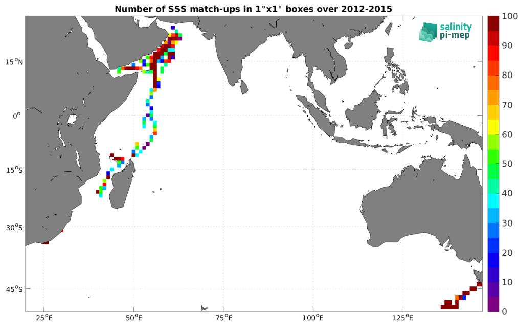
Figure 4: Number of SSS match-ups between TSG (GOSUD-Research-vessel) SSS and the Aquarius SSS L3 OR v5 - 7-Day running (NASA-GSFC) SSS product for the Indian Ocean Pi-MEP region over 1^\circ \times 1^\circ boxes and for the full satellite product period.
