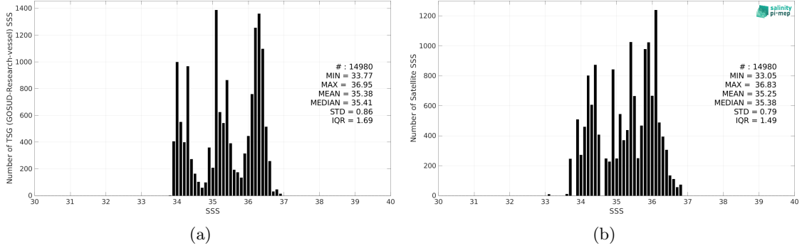
Figure 2: Histograms of SSS from TSG (GOSUD-Research-vessel) (a) and Aquarius SSS L3 OR v5 - 7-Day running (NASA-GSFC) (b) considering all match-up pairs per bins of 0.1 over the Indian Ocean Pi-MEP region and for the full satellite product period.
