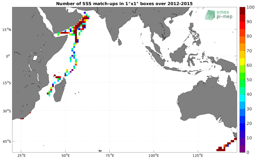
Figure 4: Number of SSS match-ups between TSG (GOSUD-Research-vessel) SSS and the Aquarius SSS L3 OR v5 - 7-Day running (NASA-GSFC) SSS product for the Indian Ocean Pi-MEP region over 1^{\circ} \times 1^{\circ} boxes and for the full satellite product period.
