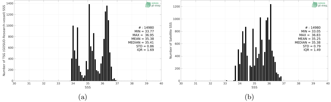
Figure 2: Histograms of SSS from TSG (GOSUD-Research-vessel) (a) and Aquarius SSS L3 OR v5 - 7-Day running (NASA-GSFC) (b) considering all match-up pairs per bins of 0.1 over the Indian Ocean Pi-MEP region and for the full satellite product period.
