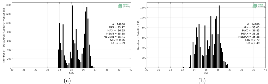
Figure 2: Histograms of SSS from TSG-GOSUD-Research-vessel (a) and Aquarius-L3-OR-V5-7DAY-RUNNING-1DEG (b) considering all match-up pairs per bins of 0.1 over the Indian Ocean Pi-MEP region and for the full satellite product period.
