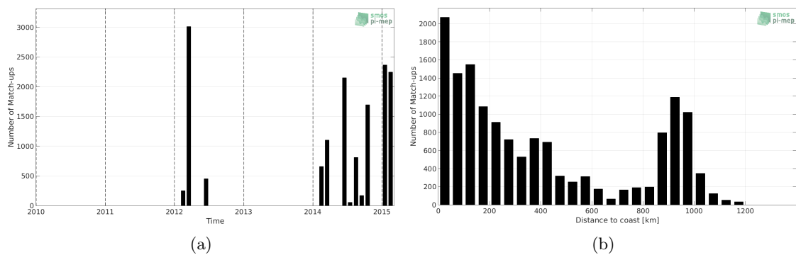
Figure 1: Number of match-ups between TSG-GOSUD-Research-vessel and Aquarius-L3-OR-V5-7DAY-RUNNING-1DEG SSS as a function of time (a) and as function of the distance to coast (b) over the Indian Ocean Pi-MEP region and for the full satellite product period.
