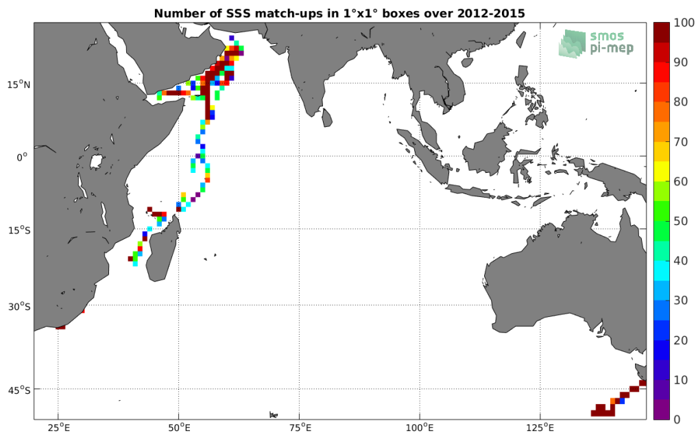
Figure 4: Number of SSS match-ups between TSG-GOSUD-Research-vessel SSS and the Aquarius-L3-OR-V5-7DAY-RUNNING-1DEG SSS product for the Indian Ocean Pi-MEP region over 1^\circ \times 1^\circ boxes and for the full satellite product period.
