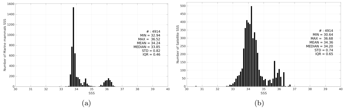
Figure 3: Histograms of SSS from Marine mammals (a) and Aquarius SSS L3 OR v5 - 7-Day running (NASA-GSFC) (b) considering all match-up pairs per bins of 0.1 over the Indian Ocean Pi-MEP region and for the full satellite product period.
