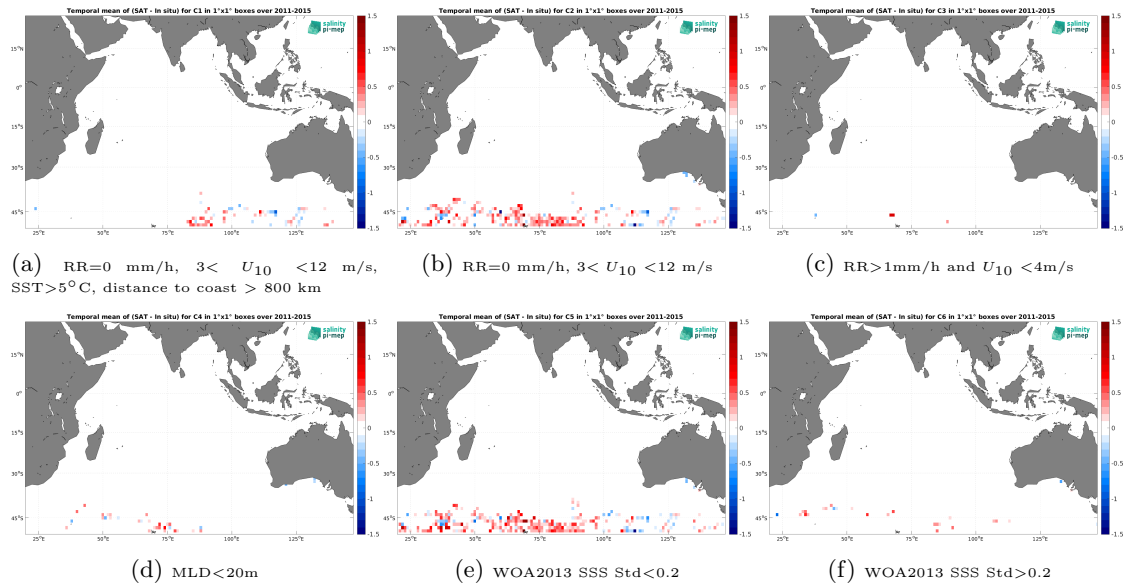
Figure 14: Temporal mean gridded over spatial boxes of size 1^\circ \times 1^\circ of \Delta SSS (Aquarius SSS L3 OR v5 - 7-Day running (NASA-GSFC) - Marine mammals) for 6 different subdatasets corresponding to:RR=0 mm/h, 3 < U_{10} < 12 m/s, SST >5^\circ C, distance to coast > 800 km (a), RR=0 mm/h, 3 < U_{10} < 12 m/s (b), RR >1 mm/h and U_{10} < 4 m/s (c),MLD <20 m (d),WOA2013 SSS Std <0.2 (e),WOA2013 SSS Std >0.2 (f).
