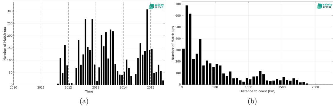
Figure 2: Number of match-ups between Marine mammals and Aquarius SSS L3 OR v5 - 7-Day running (NASA-GSFC) SSS as a function of time (a) and as function of the distance to coast (b) over the Indian Ocean Pi-MEP region and for the full satellite product period.
