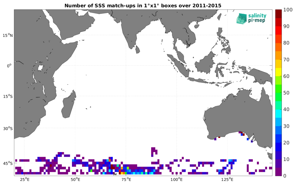
Figure 5: Number of SSS match-ups between Marine mammals SSS and the Aquarius SSS L3 OR v5 - 7-Day running (NASA-GSFC) SSS product for the Indian Ocean Pi-MEP region over 1^\circ \times 1^\circ boxes and for the full satellite product period.
