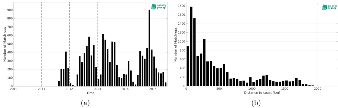
Figure 1: Number of match-ups between Marine mammals and Aquarius SSS L3 OR v5 - 7-Day running (NASA-GSFC) SSS as a function of time (a) and as function of the distance to coast (b) over the Indian Ocean Pi-MEP region and for the full satellite product period.
