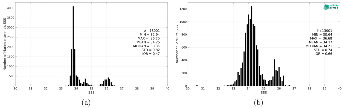
Figure 2: Histograms of SSS from Marine mammals (a) and Aquarius SSS L3 OR v5 - 7-Day running (NASA-GSFC) (b) considering all match-up pairs per bins of 0.1 over the Indian Ocean Pi-MEP region and for the full satellite product period.
