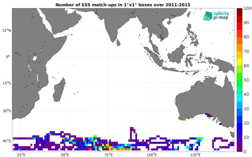
Figure 4: Number of SSS match-ups between Marine mammals SSS and the Aquarius SSS L3 OR v5 - 7-Day running (NASA-GSFC) SSS product for the Indian Ocean Pi-MEP region over 1^\circ \times 1^\circ boxes and for the full satellite product period.
