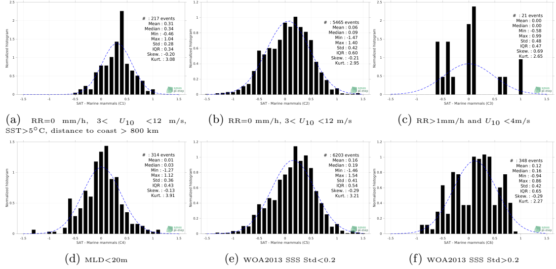
Figure 13: Normalized histogram of \Delta SSS (Aquarius SSS L3 OR v5 - 7-Day running (NASA-GSFC) - Marine mammals) for 6 different subdatasets corresponding to: RR=0 mm/h, 3 < U_{10} < 12 m/s, SST>5°C, distance to coast > 800 km (a), RR=0 mm/h, 3 < U_{10} < 12 m/s (b), RR>1mm/h and U_{10} < 4 m/s (c), MLD<20m (d), WOA2013 SSS Std<0.2 (e), WOA2013 SSS Std>0.2 (f).
