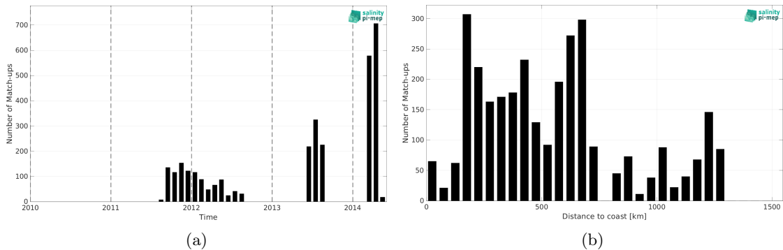
Figure 2: Number of match-ups between Surface drifters and Aquarius SSS L3 OR v5 - 7-Day running (NASA-GSFC) SSS as a function of time (a) and as function of the distance to coast (b) over the Indian Ocean Pi-MEP region and for the full satellite product period.
