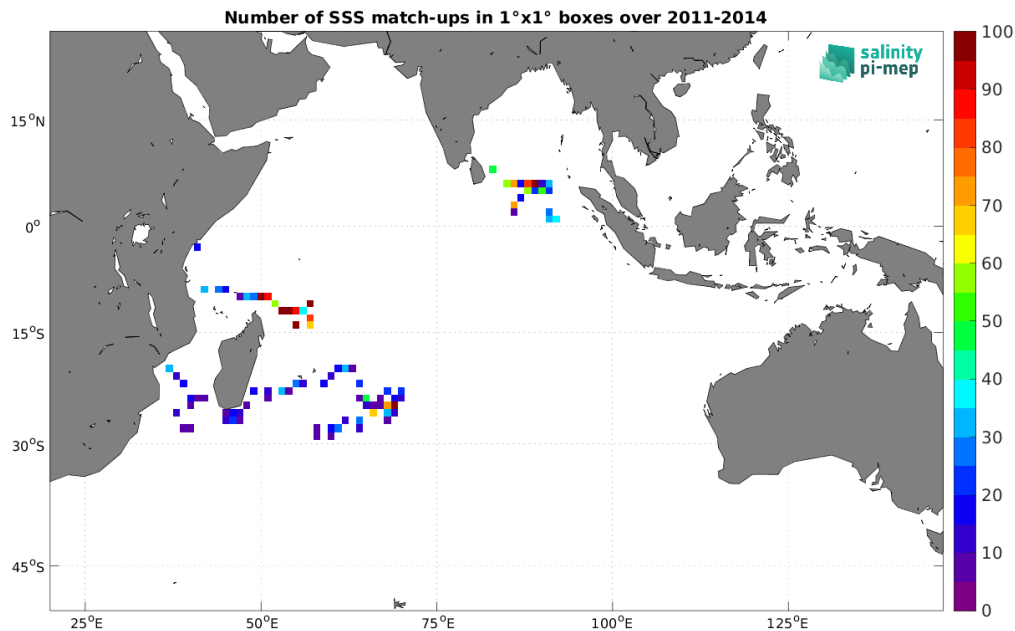
Figure 4: Number of SSS match-ups between Surface drifters SSS and the Aquarius SSS L3 OR v5 - 7-Day running (NASA-GSFC) SSS product for the Indian Ocean Pi-MEP region over 1^\circ \times 1^\circ boxes and for the full satellite product period.
