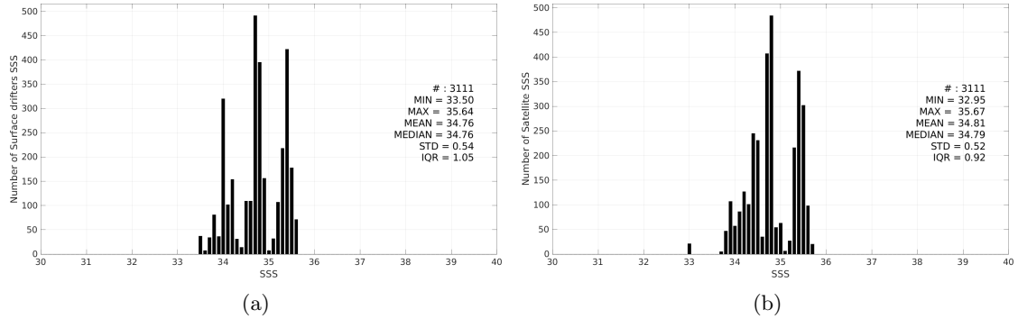
Figure 3: Histograms of SSS from Surface drifters (a) and Aquarius SSS L3 OR v5 - 7-Day running (NASA-GSFC) (b) considering all match-up pairs per bins of 0.1 over the Indian Ocean Pi-MEP region and for the full satellite product period.
