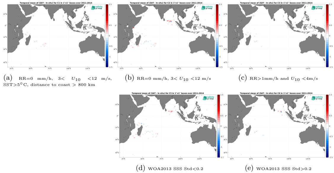
Figure 13: Temporal mean gridded over spatial boxes of size 1^\circ \times 1^\circ of \Delta SSS (Aquarius SSS L3 OR v5 - 7-Day running (NASA-GSFC) - Surface drifters) for 5 different subdatasets corresponding to: RR=0 mm/h, 3 < U_{10} < 12 m/s, SST > 5^\circ\text{C} , distance to coast > 800 km (a), RR=0 mm/h, 3 < U_{10} < 12 m/s (b), RR > 1\text{mm/h} and U_{10} < 4\text{m/s} (c), WOA2013 SSS Std < 0.2 (d), WOA2013 SSS Std > 0.2 (e).
