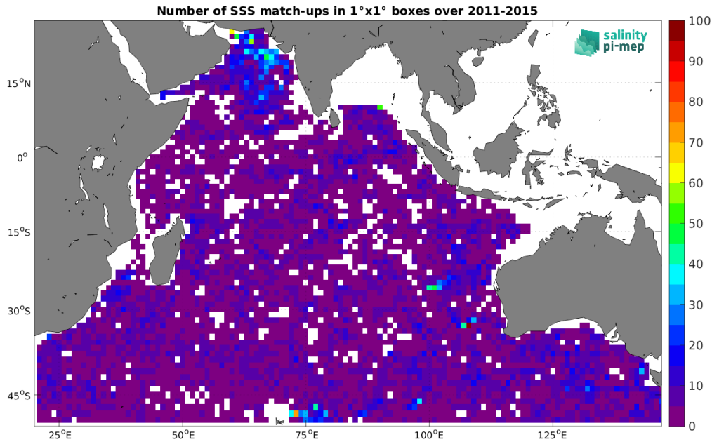
Figure 5: Number of SSS match-ups between Argo SSS and the Aquarius SSS L3 OR v5 - 7-Day running (NASA-GSFC) SSS product for the Indian Ocean Pi-MEP region over 1^\circ \times 1^\circ boxes and for the full satellite product period.
