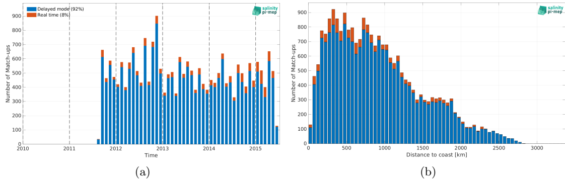
Figure 2: Number of match-ups between Argo and Aquarius SSS L3 OR v5 - 7-Day running (NASA-GSFC) SSS as a function of time (a) and as function of the distance to coast (b) over the Indian Ocean Pi-MEP region and for the full satellite product period.
