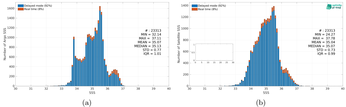
Figure 3: Histograms of SSS from Argo (a) and Aquarius SSS L3 OR v5 - 7-Day running (NASA-GSFC) (b) considering all match-up pairs per bins of 0.1 over the Indian Ocean Pi-MEP region and for the full satellite product period.
