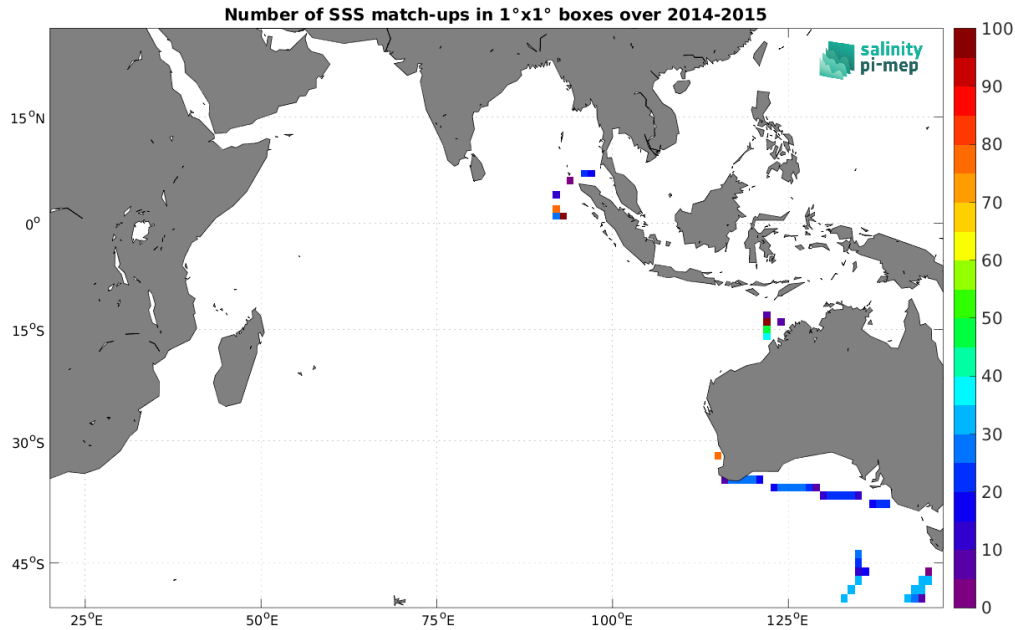
Figure 5: Number of SSS match-ups between TSG (SAMOS) SSS and the Aquarius SSS L3 OR v5 - 7-Day running - Rain mask (NASA-GSFC) SSS product for the Indian Ocean Pi-MEP region over 1^\circ \times 1^\circ boxes and for the full satellite product period.
