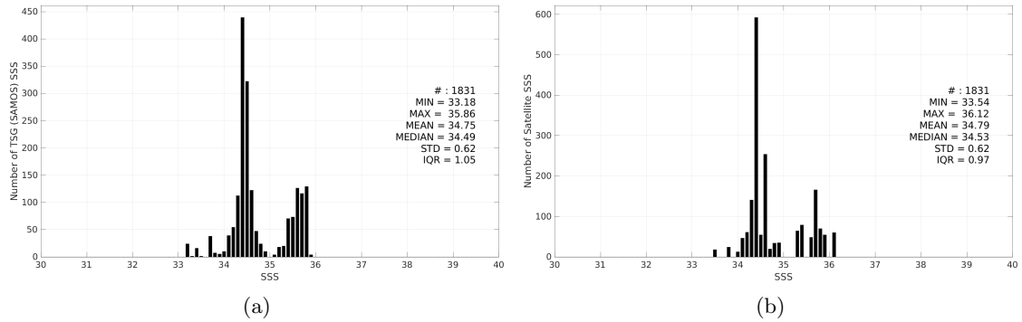
Figure 3: Histograms of SSS from TSG (SAMOS) (a) and Aquarius SSS L3 OR v5 - 7-Day running - Rain mask (NASA-GSFC) (b) considering all match-up pairs per bins of 0.1 over the Indian Ocean Pi-MEP region and for the full satellite product period.
