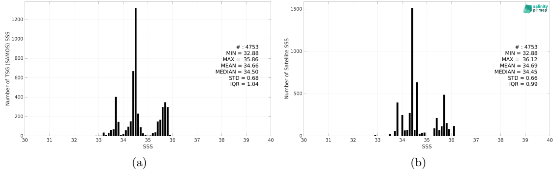
Figure 2: Histograms of SSS from TSG (SAMOS) (a) and Aquarius SSS L3 OR v5 - 7-Day running - Rain mask (NASA-GSFC) (b) considering all match-up pairs per bins of 0.1 over the Indian Ocean Pi-MEP region and for the full satellite product period.
