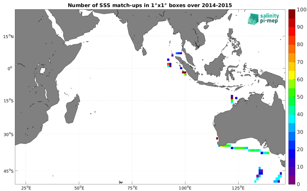
Figure 4: Number of SSS match-ups between TSG (SAMOS) SSS and the Aquarius SSS L3 OR v5 - 7-Day running - Rain mask (NASA-GSFC) SSS product for the Indian Ocean Pi-MEP region over 1^\circ \times 1^\circ boxes and for the full satellite product period.
