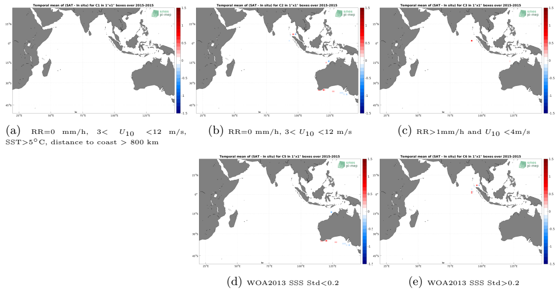
Figure 12: Temporal mean gridded over spatial boxes of size 1^{\circ}\times 1^{\circ} of \Delta\text{SSS} (Aquarius SSS L3 OR v5 - 7-Day running - Rain mask (NASA-GSFC) - TSG (SAMOS)) for 5 different subdatasets corresponding to:RR=0 mm/h, 3 < U_{10} < 12 m/s, SST >5^{\circ}\text{C} , distance to coast > 800 km (a), RR=0 mm/h, 3 < U_{10} < 12 m/s (b), RR >1 mm/h and U_{10} < 4 m/s (c), WOA2013 SSS Std <0.2 (d), WOA2013 SSS Std >0.2 (e).
