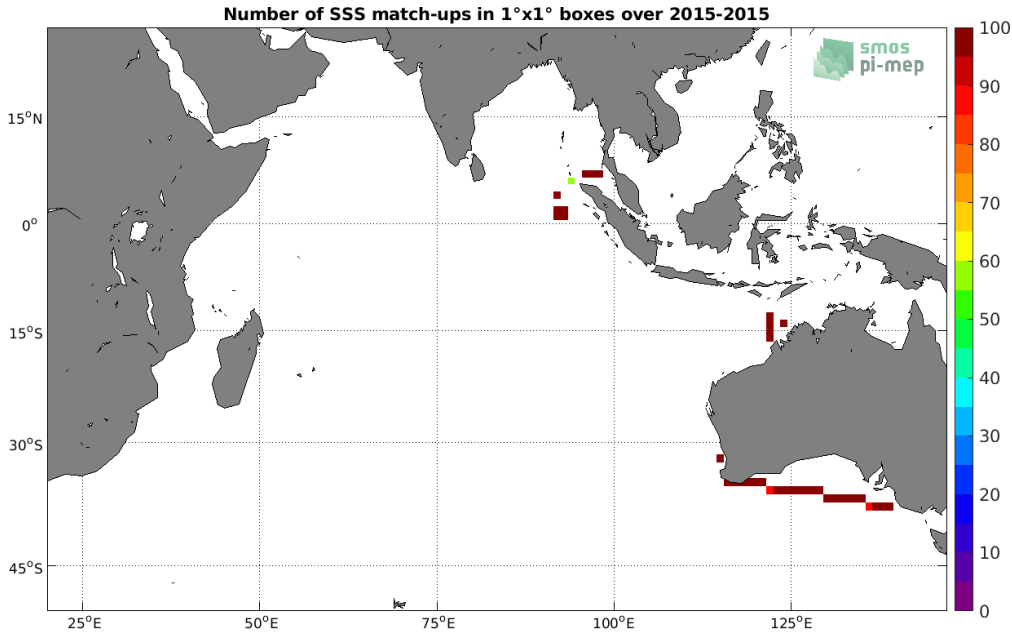
Figure 4: Number of SSS match-ups between TSG (SAMOS) SSS and the Aquarius SSS L3 OR v5 - 7-Day running - Rain mask (NASA-GSFC) SSS product for the Indian Ocean Pi-MEP region over 1°x1° boxes and for the full satellite product period.
