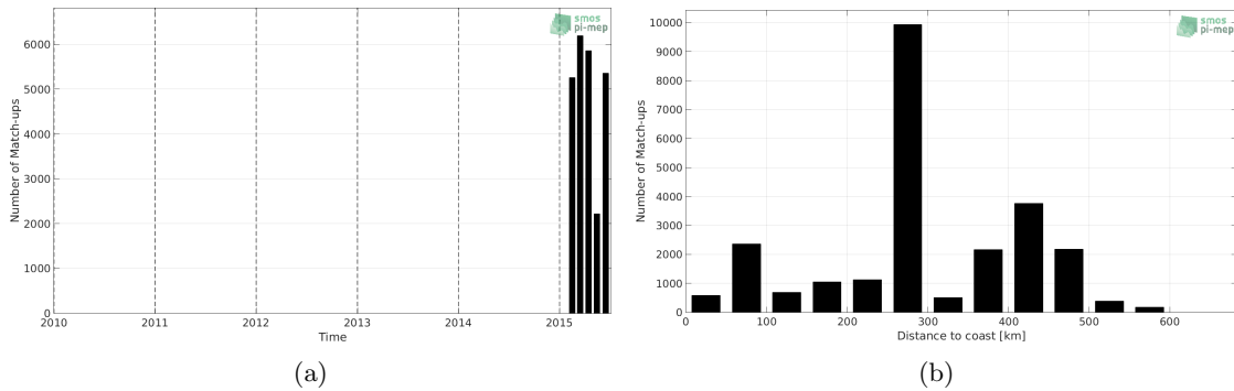
Figure 1: Number of match-ups between TSG-SAMOS and Aquarius-L3-OR-V5-7DAY-RUNNING-RAIN-MASK-1DEG SSS as a function of time (a) and as function of the distance to coast (b) over the Indian Ocean Pi-MEP region and for the full satellite product period.
