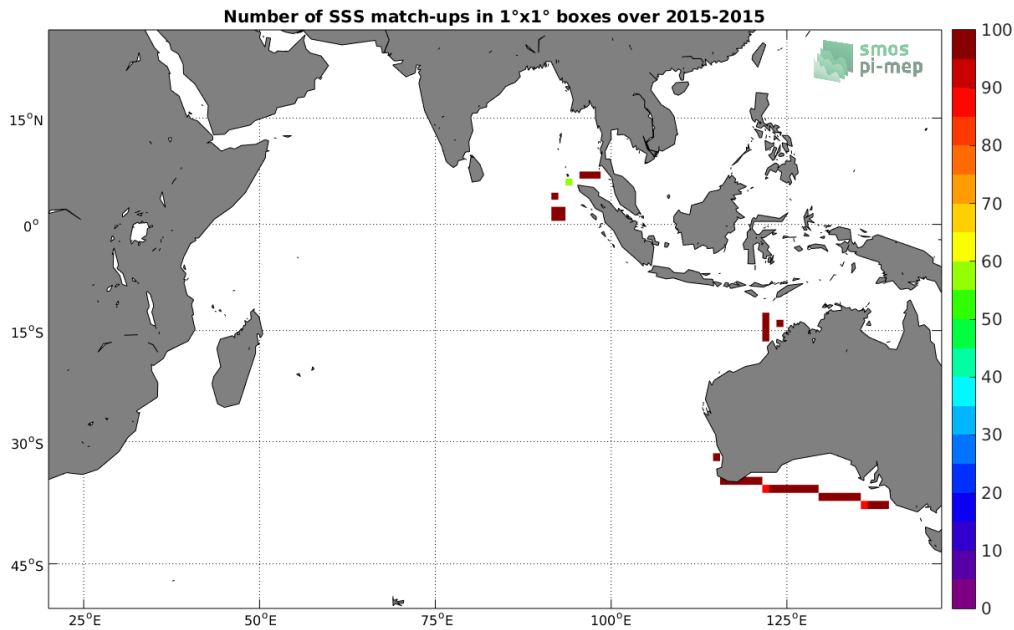
Figure 4: Number of SSS match-ups between TSG-SAMOS SSS and the Aquarius-L3-OR-V5-7DAY-RUNNING-RAIN-MASK-1DEG SSS product for the Indian Ocean Pi-MEP region over 1^\circ \times 1^\circ boxes and for the full satellite product period.
