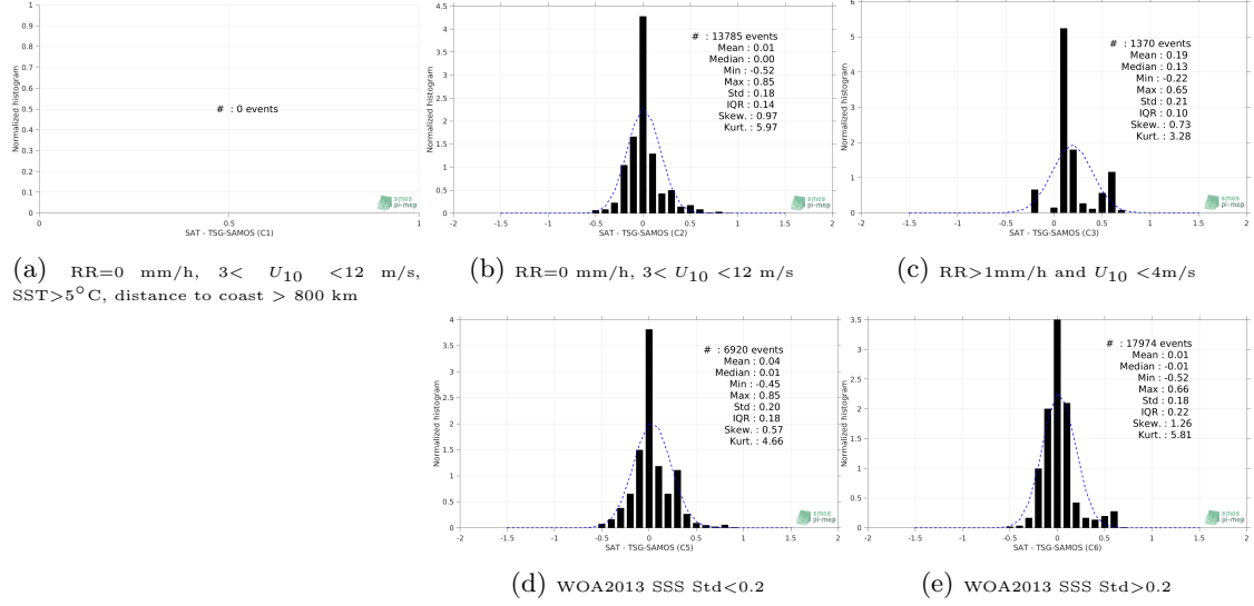
Figure 13: Normalized histogram of \Delta\text{SSS} (Aquarius-L3-OR-V5-7DAY-RUNNING-RAIN-MASK-1DEG - TSG-SAMOS) for 5 different subdatasets corresponding to: RR=0 mm/h, 3 < U_{10} < 12 m/s, SST > 5^{\circ}\text{C} , distance to coast > 800 km (a), RR=0 mm/h, 3 < U_{10} < 12 m/s (b), RR > 1\text{mm/h} and U_{10} < 4\text{m/s} (c), WOA2013 SSS Std < 0.2 (d), WOA2013 SSS Std > 0.2 (e).
