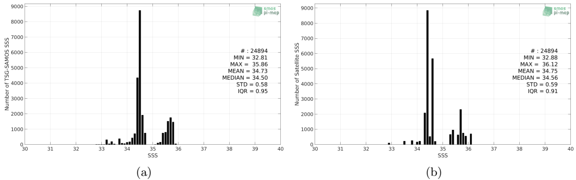
Figure 2: Histograms of SSS from TSG-SAMOS (a) and Aquarius-L3-OR-V5-7DAY-RUNNING-RAIN-MASK-1DEG (b) considering all match-up pairs per bins of 0.1 over the Indian Ocean Pi-MEP region and for the full satellite product period.
