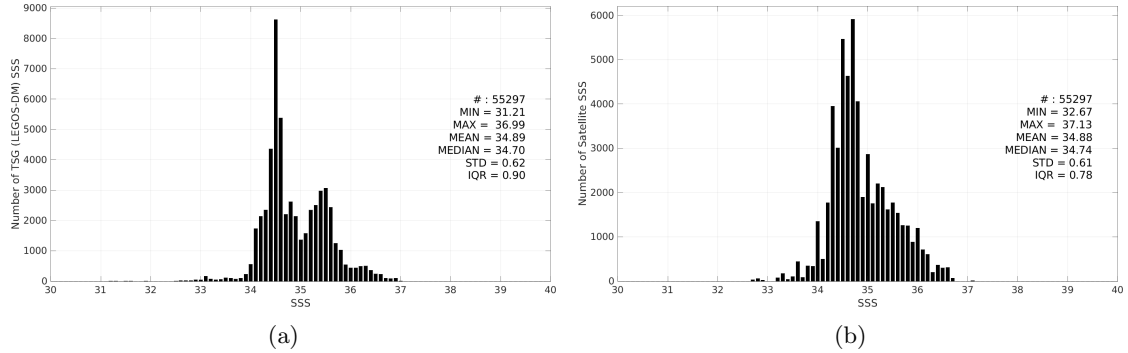
Figure 3: Histograms of SSS from TSG (LEGOS-DM) (a) and Aquarius SSS L3 OR v5 - 7-Day running - Rain mask (NASA-GSFC) (b) considering all match-up pairs per bins of 0.1 over the Indian Ocean Pi-MEP region and for the full satellite product period.
