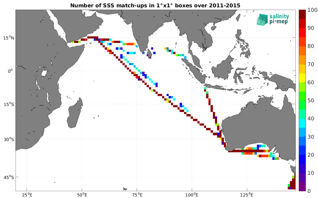
Figure 5: Number of SSS match-ups between TSG (LEGOS-DM) SSS and the Aquarius SSS L3 OR v5 - 7-Day running - Rain mask (NASA-GSFC) SSS product for the Indian Ocean Pi-MEP region over 1^\circ \times 1^\circ boxes and for the full satellite product period.
