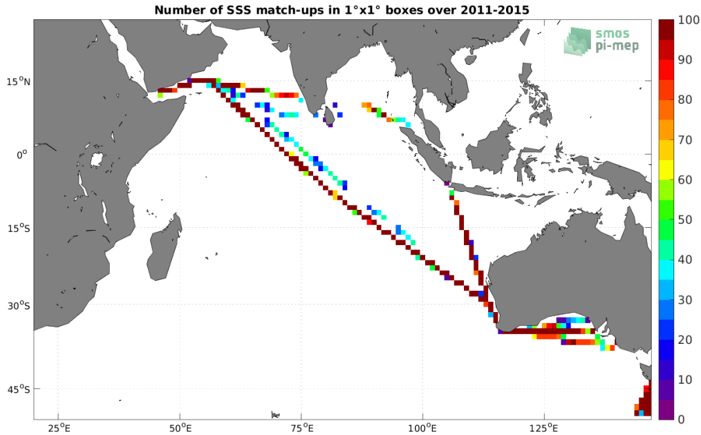
Figure 4: Number of SSS match-ups between TSG (LEGOS-DM) SSS and the Aquarius SSS L3 OR v5 - 7-Day running - Rain mask (NASA-GSFC) SSS product for the Indian Ocean Pi-MEP region over 1^\circ \times 1^\circ boxes and for the full satellite product period.
