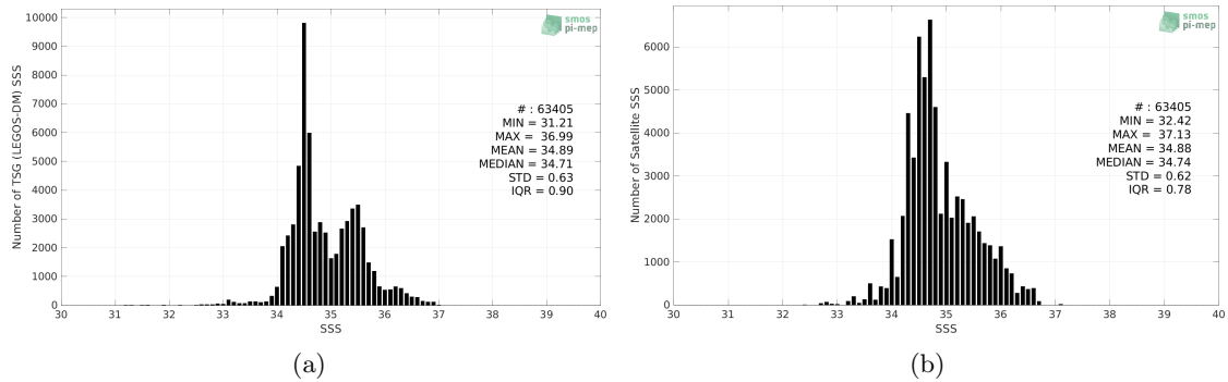
Figure 2: Histograms of SSS from TSG (LEGOS-DM) (a) and Aquarius SSS L3 OR v5 - 7-Day running - Rain mask (NASA-GSFC) (b) considering all match-up pairs per bins of 0.1 over the Indian Ocean Pi-MEP region and for the full satellite product period.
