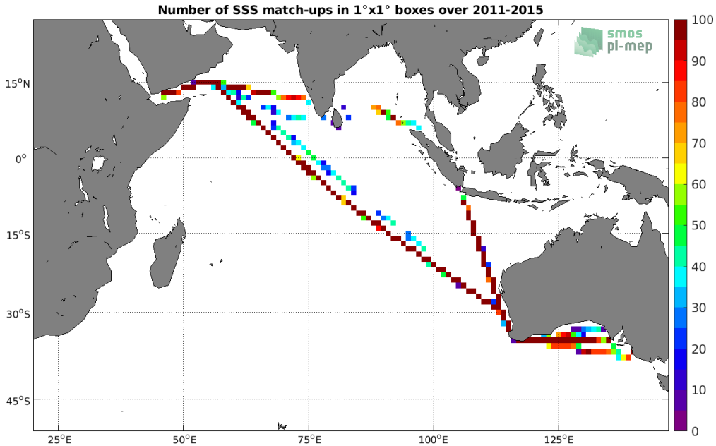
Figure 4: Number of SSS match-ups between TSG (LEGOS-DM) SSS and the Aquarius SSS L3 OR v5 - 7-Day running - Rain mask (NASA-GSFC) SSS product for the Indian Ocean Pi-MEP region over 1^\circ \times 1^\circ boxes and for the full satellite product period.
