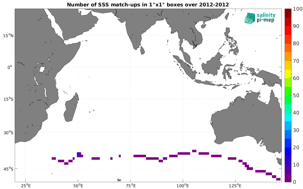
Figure 5: Number of SSS match-ups between TSG (GOSUD-Sailing-ship) SSS and the Aquarius SSS L3 OR v5 - 7-Day running - Rain mask (NASA-GSFC) SSS product for the Indian Ocean Pi-MEP region over 1^\circ \times 1^\circ boxes and for the full satellite product period.
