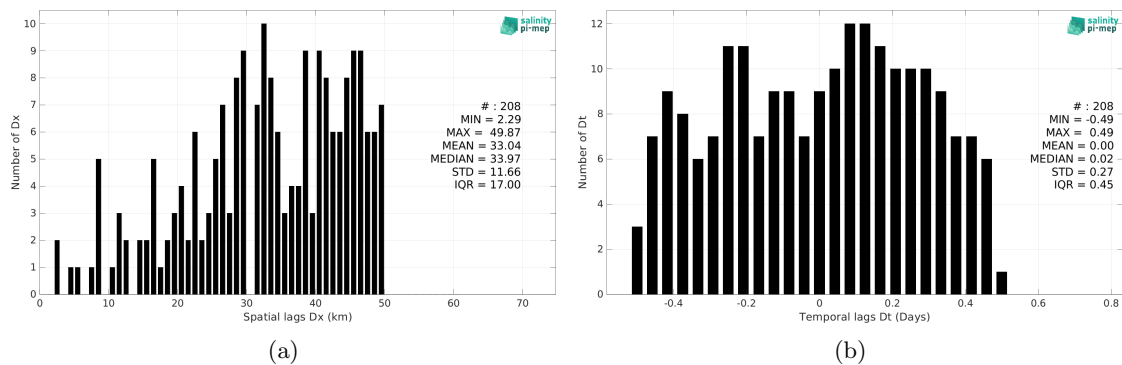
Figure 6: Histograms of the spatial (a) and temporal (b) lags between the location/time of the TSG (GOSUD-Sailing-ship) measurement and the date of the corresponding Aquarius SSS L3 OR v5 - 7-Day running - Rain mask (NASA-GSFC) SSS pixel.
