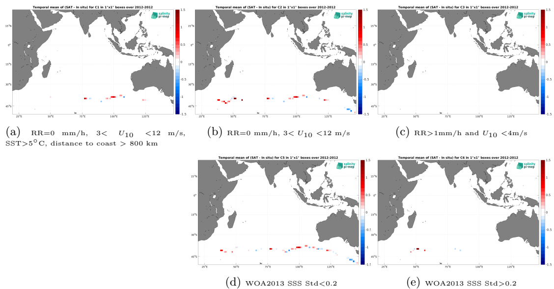
Figure 14: Temporal mean gridded over spatial boxes of size 1^\circ \times 1^\circ of \Delta SSS (Aquarius SSS L3 OR v5 - 7-Day running - Rain mask (NASA-GSFC) - TSG (GOSUD-Sailing-ship)) for 5 different subdatasets corresponding to:RR=0 mm/h, 3 < U_{10} < 12 m/s, SST > 5^\circ\text{C} , distance to coast > 800 km (a), RR=0 mm/h, 3 < U_{10} < 12 m/s (b), RR > 1 mm/h and U_{10} < 4 m/s (c), WOA2013 SSS Std < 0.2 (d), WOA2013 SSS Std > 0.2 (e).
