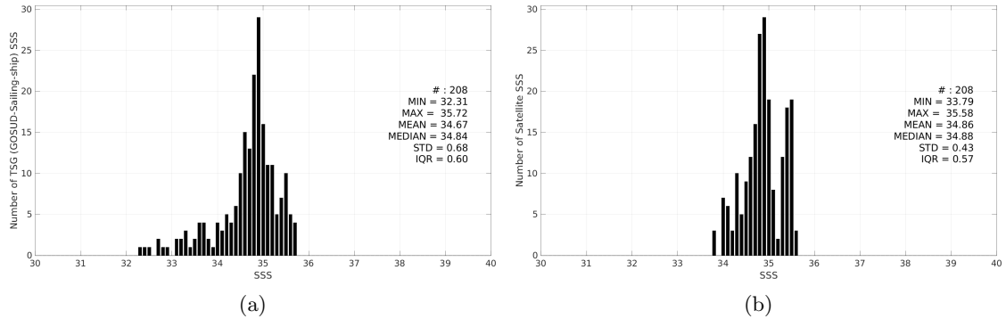
Figure 3: Histograms of SSS from TSG (GOSUD-Sailing-ship) (a) and Aquarius SSS L3 OR v5 - 7-Day running - Rain mask (NASA-GSFC) (b) considering all match-up pairs per bins of 0.1 over the Indian Ocean Pi-MEP region and for the full satellite product period.
