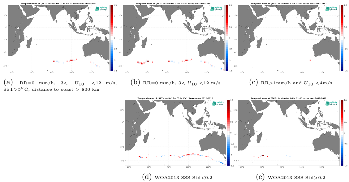
Figure 12: Temporal mean gridded over spatial boxes of size 1^{\circ}\times 1^{\circ} of \Delta SSS (Aquarius SSS L3 OR v5 - 7-Day running - Rain mask (NASA-GSFC) - TSG (GOSUD-Sailing-ship)) for 5 different subdatasets corresponding to:RR=0 mm/h, 3 < U_{10} < 12 m/s, SST >5^{\circ}\text{C} , distance to coast > 800 km (a), RR=0 mm/h, 3 < U_{10} < 12 m/s (b), RR >1 mm/h and U_{10} < 4 m/s (c), WOA2013 SSS Std <0.2 (d), WOA2013 SSS Std >0.2 (e).
