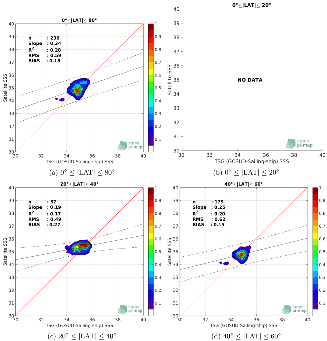
Figure 9: Contour maps of the concentration of Aquarius SSS L3 OR v5 - 7-Day running - Rain mask (NASA-GSFC) SSS ( y -axis) versus TSG (GOSUD-Sailing-ship) SSS ( x -axis) at match-up pairs for different latitude bands. For each plot, the red line shows x=y . The black thin and dashed lines indicate a linear fit through the data cloud and the \pm 95\% confidence levels, respectively. The number match-up pairs n , the slope and R^2 coefficient of the linear fit, the root mean square (RMS) and the mean bias between satellite and in situ data are indicated for each latitude band in each plots.
