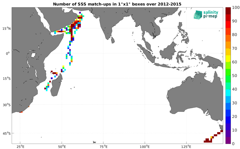
Figure 5: Number of SSS match-ups between TSG (GOSUD-Research-vessel) SSS and the Aquarius SSS L3 OR v5 - 7-Day running - Rain mask (NASA-GSFC) SSS product for the Indian Ocean Pi-MEP region over 1^\circ \times 1^\circ boxes and for the full satellite product period.
