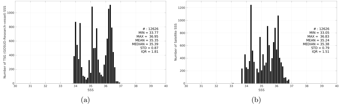
Figure 3: Histograms of SSS from TSG (GOSUD-Research-vessel) (a) and Aquarius SSS L3 OR v5 - 7-Day running - Rain mask (NASA-GSFC) (b) considering all match-up pairs per bins of 0.1 over the Indian Ocean Pi-MEP region and for the full satellite product period.
