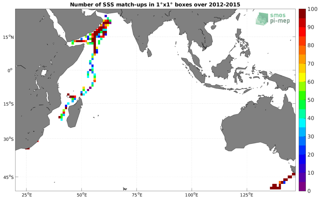
Figure 4: Number of SSS match-ups between TSG (GOSUD-Research-vessel) SSS and the Aquarius SSS L3 OR v5 - 7-Day running - Rain mask (NASA-GSFC) SSS product for the Indian Ocean Pi-MEP region over 1^\circ \times 1^\circ boxes and for the full satellite product period.
