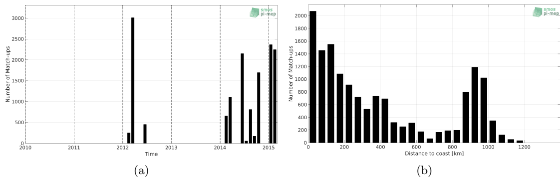
Figure 1: Number of match-ups between TSG-GOSUD-Research-vessel and Aquarius-L3-OR-V5-7DAY-RUNNING-RAIN-MASK-1DEG SSS as a function of time (a) and as function of the distance to coast (b) over the Indian Ocean Pi-MEP region and for the full satellite product period.
