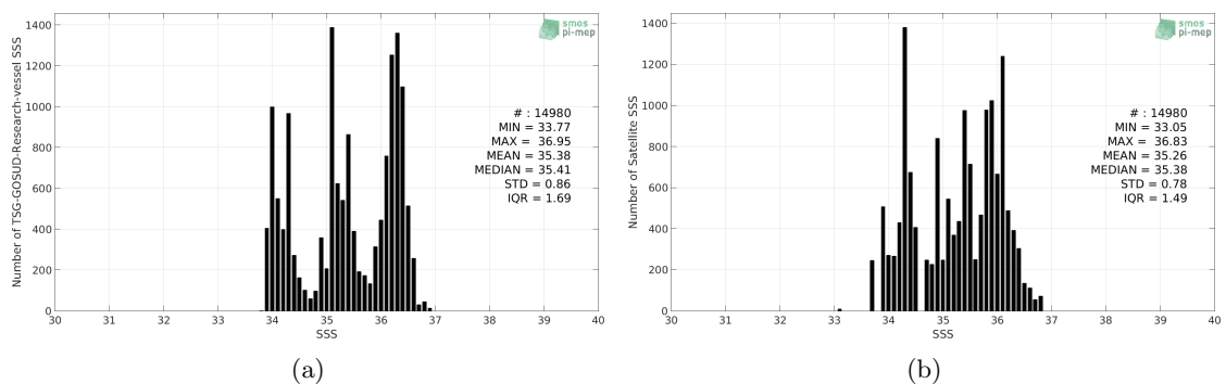
Figure 2: Histograms of SSS from TSG-GOSUD-Research-vessel (a) and Aquarius-L3-OR-V5-7DAY-RUNNING-RAIN-MASK-1DEG (b) considering all match-up pairs per bins of 0.1 over the Indian Ocean Pi-MEP region and for the full satellite product period.
