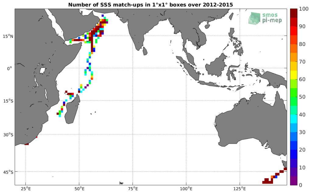
Figure 4: Number of SSS match-ups between TSG-GOSUD-Research-vessel SSS and the Aquarius-L3-OR-V5-7DAY-RUNNING-RAIN-MASK-1DEG SSS product for the Indian Ocean Pi-MEP region over 1°x1° boxes and for the full satellite product period.
