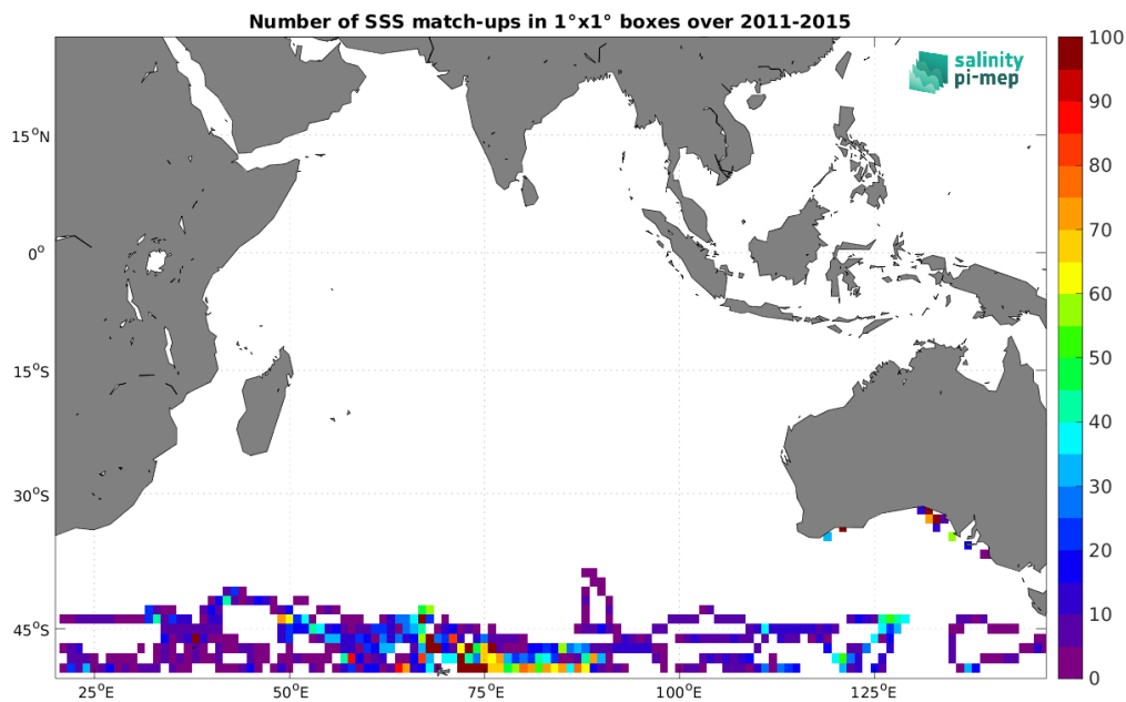
Figure 5: Number of SSS match-ups between Marine mammals SSS and the Aquarius SSS L3 OR v5 - 7-Day running - Rain mask (NASA-GSFC) SSS product for the Indian Ocean Pi-MEP region over 1^\circ \times 1^\circ boxes and for the full satellite product period.
