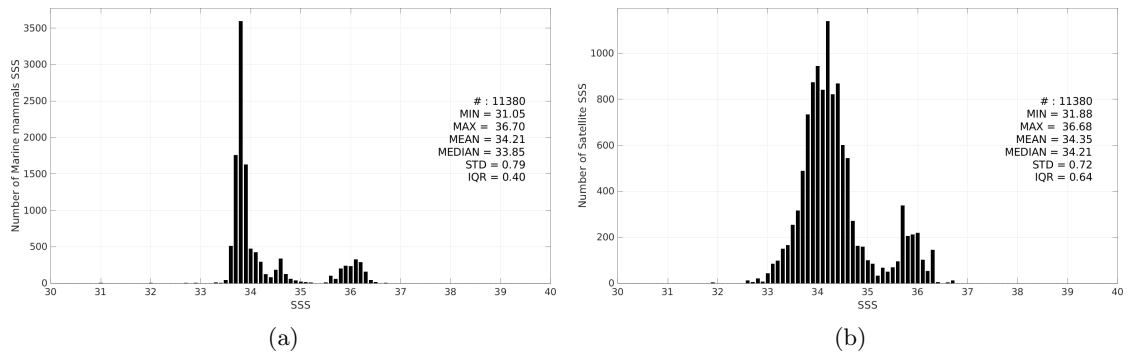
Figure 3: Histograms of SSS from Marine mammals (a) and Aquarius SSS L3 OR v5 - 7-Day running - Rain mask (NASA-GSFC) (b) considering all match-up pairs per bins of 0.1 over the Indian Ocean Pi-MEP region and for the full satellite product period.
