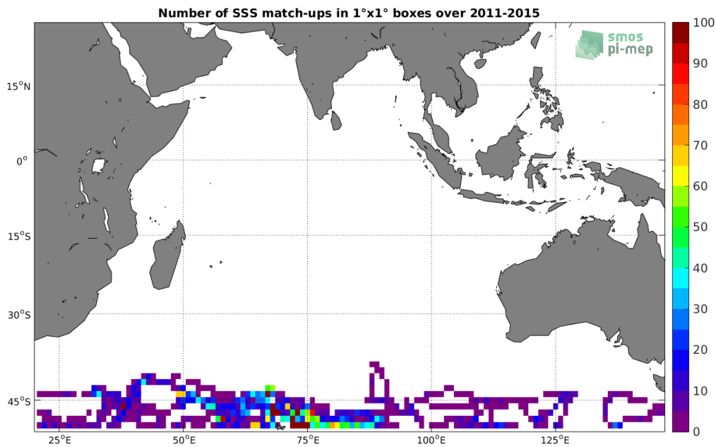
Figure 4: Number of SSS match-ups between Sea mammals SSS and the Aquarius-L3-OR-V5-7DAY-RUNNING-RAIN-MASK-1DEG SSS product for the Indian Ocean Pi-MEP region over 1^\circ \times 1^\circ boxes and for the full satellite product period.
