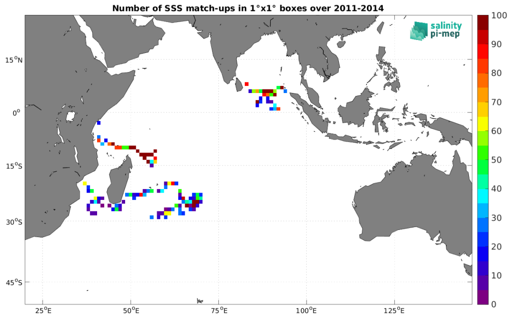
Figure 4: Number of SSS match-ups between Surface drifters SSS and the Aquarius SSS L3 OR v5 - 7-Day running - Rain mask (NASA-GSFC) SSS product for the Indian Ocean Pi-MEP region over 1^\circ \times 1^\circ boxes and for the full satellite product period.
