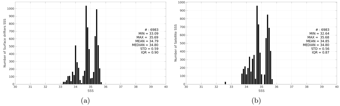
Figure 3: Histograms of SSS from Surface drifters (a) and Aquarius SSS L3 OR v5 - 7-Day running - Rain mask (NASA-GSFC) (b) considering all match-up pairs per bins of 0.1 over the Indian Ocean Pi-MEP region and for the full satellite product period.
