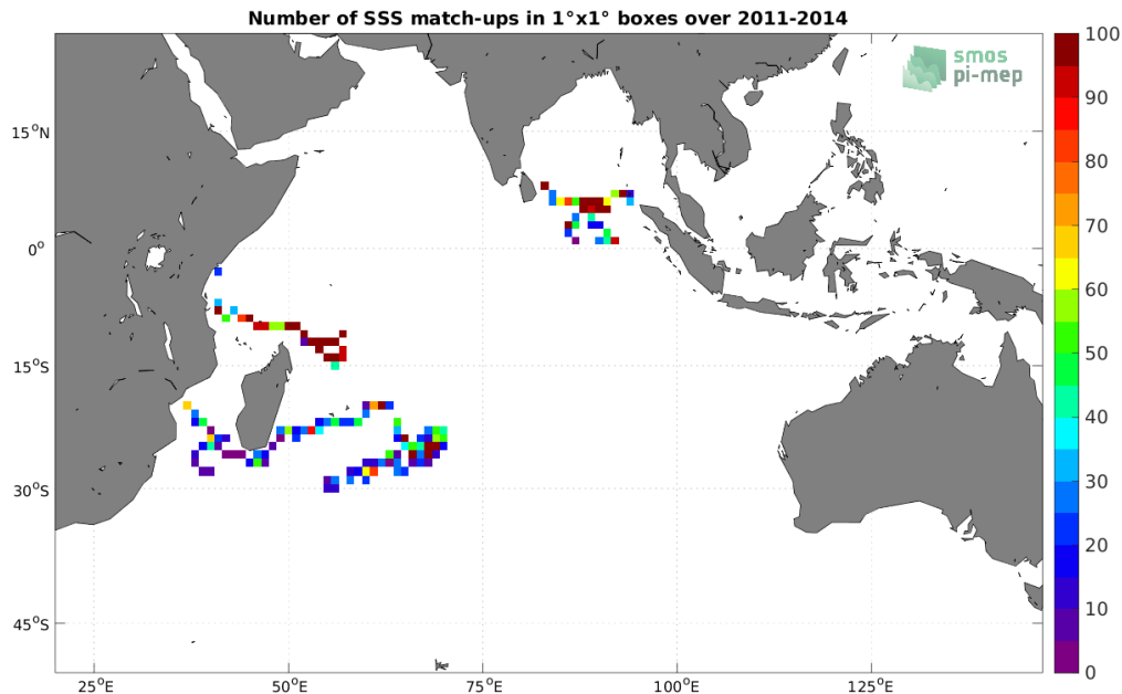
Figure 3: Number of SSS match-ups between Surface drifters SSS and the Aquarius SSS L3 OR v5 - 7-Day running - Rain mask (NASA-GSFC) SSS product for the Indian Ocean Pi-MEP region over 1^\circ \times 1^\circ boxes and for the full satellite product period.
