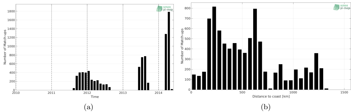
Figure 1: Number of match-ups between Surface drifters and Aquarius-L3-OR-V5-7DAY-RUNNING-RAIN-MASK-1DEG SSS as a function of time (a) and as function of the distance to coast (b) over the Indian Ocean Pi-MEP region and for the full satellite product period.
