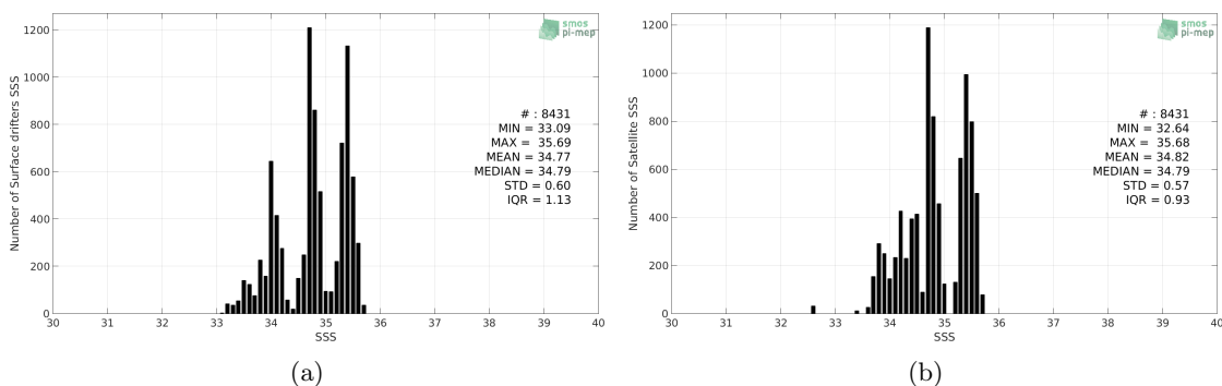
Figure 2: Histograms of SSS from Surface drifters (a) and Aquarius-L3-OR-V5-7DAY-RUNNING-RAIN-MASK-1DEG (b) considering all match-up pairs per bins of 0.1 over the Indian Ocean Pi-MEP region and for the full satellite product period.
