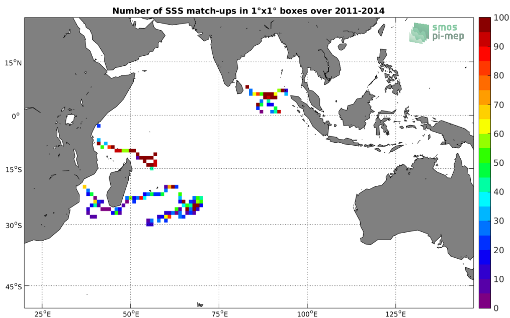
Figure 3: Number of SSS match-ups between Surface drifters SSS and the Aquarius-L3-OR-V5-7DAY-RUNNING-RAIN-MASK-1DEG SSS product for the Indian Ocean Pi-MEP region over 1°x1° boxes and for the full satellite product period.
