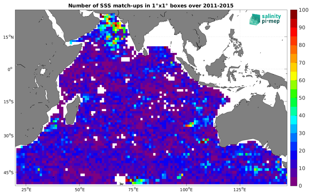
Figure 5: Number of SSS match-ups between Argo SSS and the Aquarius SSS L3 OR v5 - 7-Day running - Rain mask (NASA-GSFC) SSS product for the Indian Ocean Pi-MEP region over 1^\circ \times 1^\circ boxes and for the full satellite product period.
