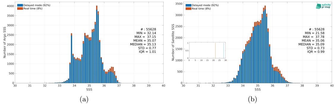
Figure 3: Histograms of SSS from Argo (a) and Aquarius SSS L3 OR v5 - 7-Day running - Rain mask (NASA-GSFC) (b) considering all match-up pairs per bins of 0.1 over the Indian Ocean Pi-MEP region and for the full satellite product period.
