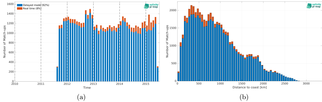
Figure 2: Number of match-ups between Argo and Aquarius SSS L3 OR v5 - 7-Day running - Rain mask (NASA-GSFC) SSS as a function of time (a) and as function of the distance to coast (b) over the Indian Ocean Pi-MEP region and for the full satellite product period.
