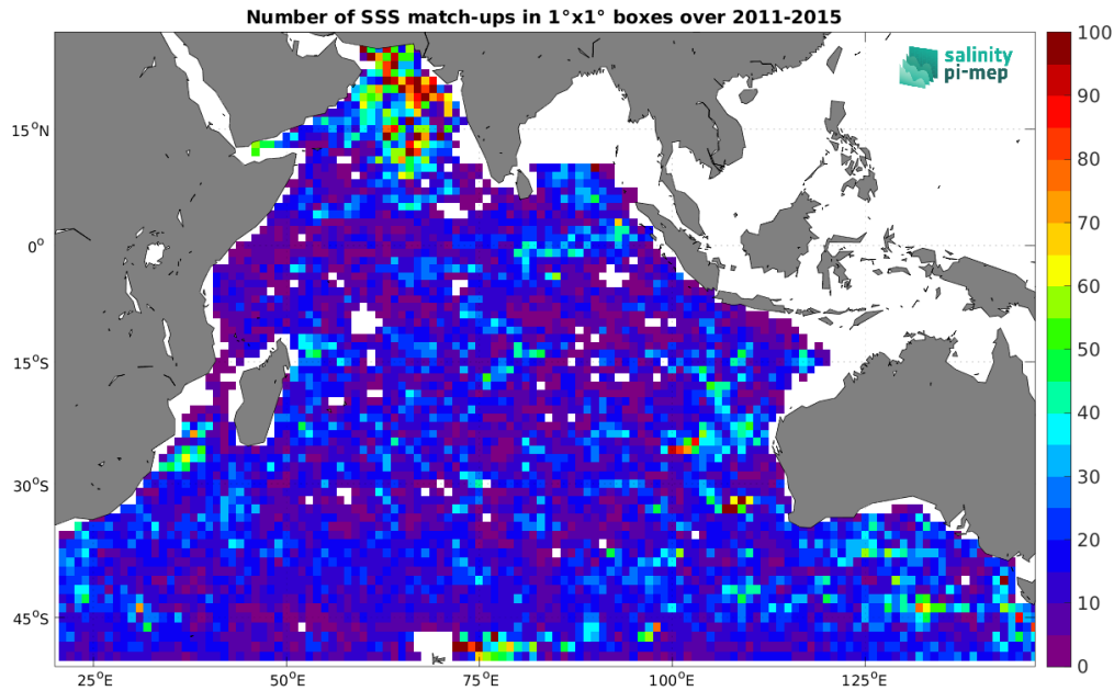
Figure 4: Number of SSS match-ups between Argo SSS and the Aquarius SSS L3 OR v5 - 7-Day running - Rain mask (NASA-GSFC) SSS product for the Indian Ocean Pi-MEP region over 1^\circ \times 1^\circ boxes and for the full satellite product period.
