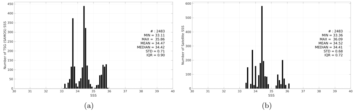
Figure 3: Histograms of SSS from TSG (SAMOS) (a) and Aquarius SSS L3 OR v5 - Monthly (NASA-GSFC) (b) considering all match-up pairs per bins of 0.1 over the Indian Ocean Pi-MEP region and for the full satellite product period.
