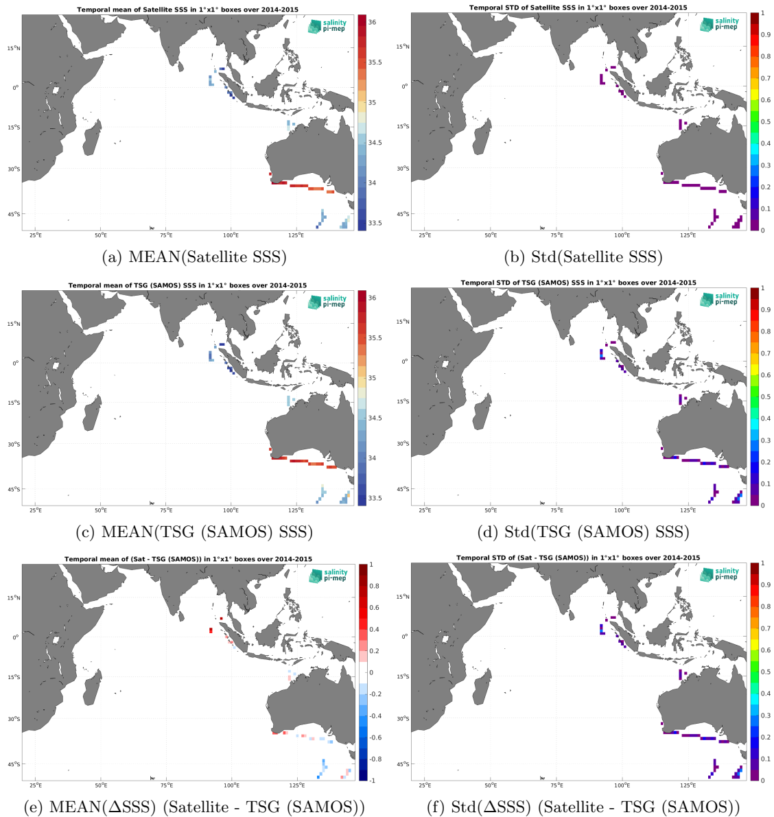
Figure 7: Temporal mean (left) and Std (right) of SSS from Aquarius SSS L3 OR v5 - Monthly (NASA-GSFC) (top), TSG (SAMOS) (middle), and of \Delta SSS (Satellite - TSG (SAMOS)). Only match-up pairs are used to generate these maps.
