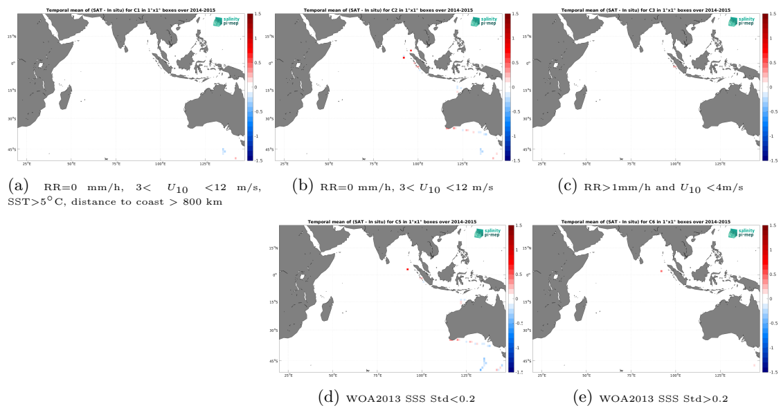
Figure 14: Temporal mean gridded over spatial boxes of size 1^\circ \times 1^\circ of \Delta SSS (Aquarius SSS L3 OR v5 - Monthly (NASA-GSFC) - TSG (SAMOS)) for 5 different subdatasets corresponding to:RR=0 mm/h, 3 < U_{10} < 12 m/s, SST >5^\circ\text{C} , distance to coast > 800 km (a), RR=0 mm/h, 3 < U_{10} < 12 m/s (b), RR >1 mm/h and U_{10} < 4 m/s (c), WOA2013 SSS Std <0.2 (d), WOA2013 SSS Std >0.2 (e).
