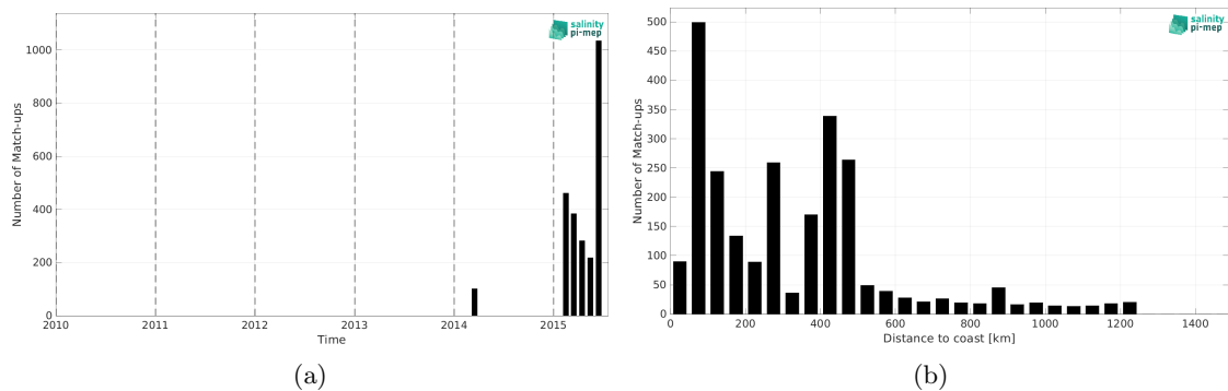
Figure 2: Number of match-ups between TSG (SAMOS) and Aquarius SSS L3 OR v5 - Monthly (NASA-GSFC) SSS as a function of time (a) and as function of the distance to coast (b) over the Indian Ocean Pi-MEP region and for the full satellite product period.
